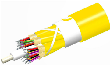
TeraSPEED® Low Smoke Zero Halogen Riser Distribution Cable, 36 fiber multi-unit with 12 fiber subunits
