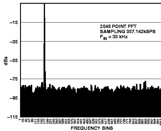
Figure 3. AD7810 SNR
