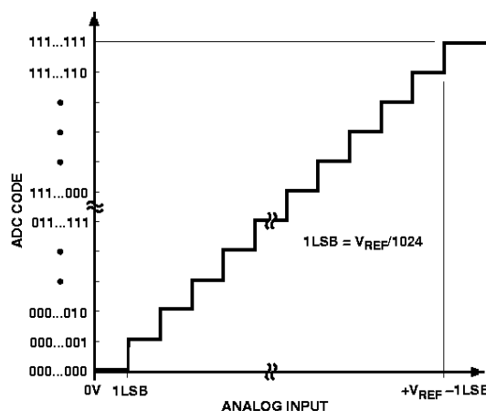
Figure 11. Transfer Characteristic
