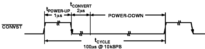
Figure 13. Automatic Power-Down
