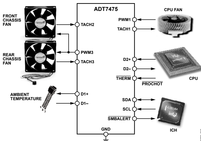
Figure 13. ADT7475 Configuration
