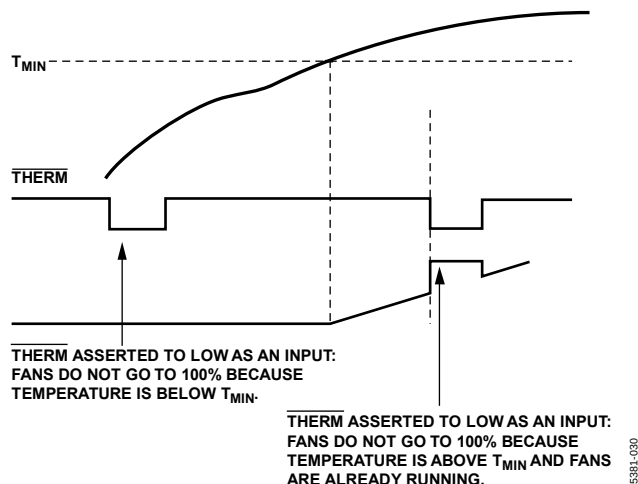
Figure 27. Asserting \overline{\text{THERM}} Low as an Input in Automatic Fan Speed Control Mode
