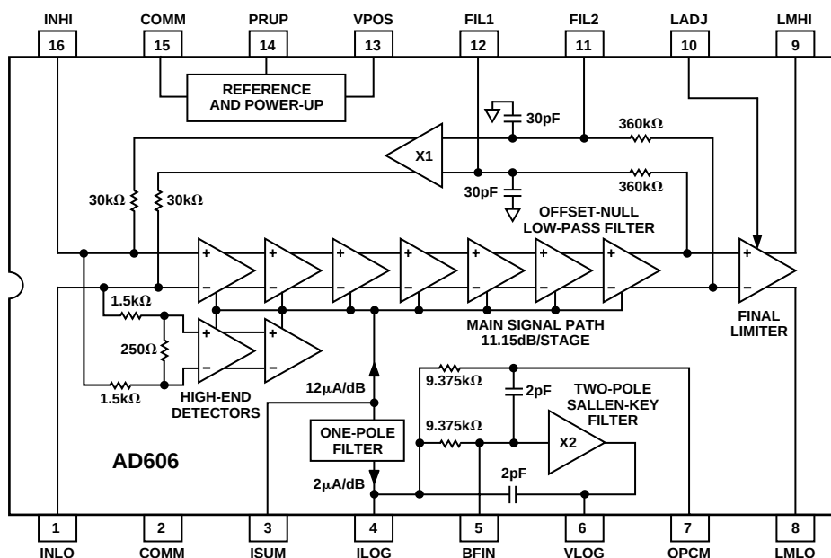
Figure 2. AD606 Simplified Block Diagram
