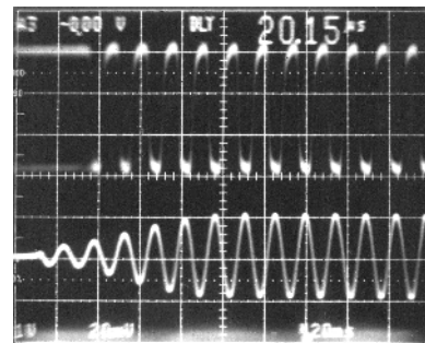
Figure 18. Limiter Response at Onset of 70 MHz Modulated Pulse at -55 dBm Using 200 pF Input Coupling Capacitors
