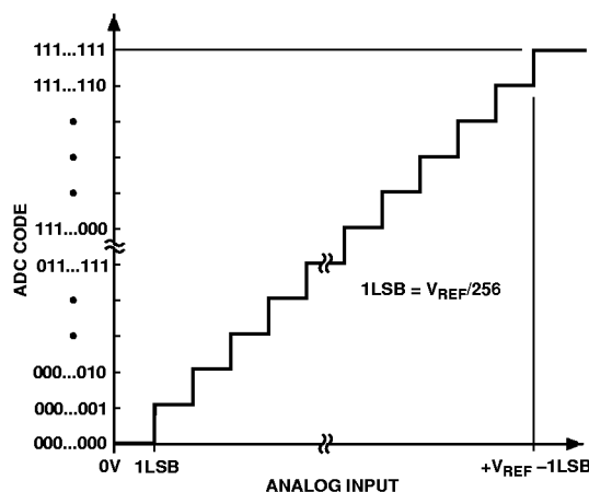
Figure 11. Transfer Characteristic
