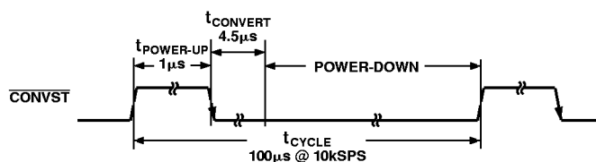
Figure 13. Automatic Power-Down
