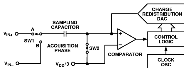
Figure 4. ADC Acquisition Phase
