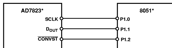
Figure 20. Interfacing to the 8051 Using I/O Ports
