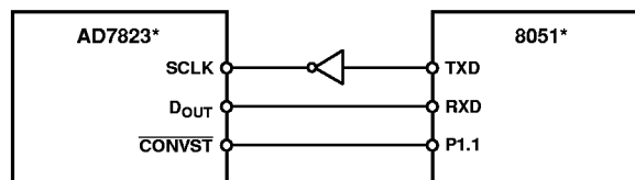
Figure 19. Interfacing to the 8051 Serial Port
