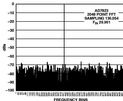
Figure 3. AD7823 SNR
