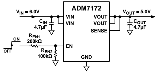
Figure 61. Typical EN Pin Voltage Divider
