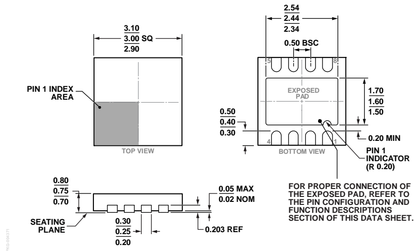
Figure 72. 8-Lead Lead Frame Chip Scale Package [LFCSP_WD] 3 mm × 3 mm Body, Very Very Thin, Dual Lead (CP-8-21) Dimensions shown in millimeters
