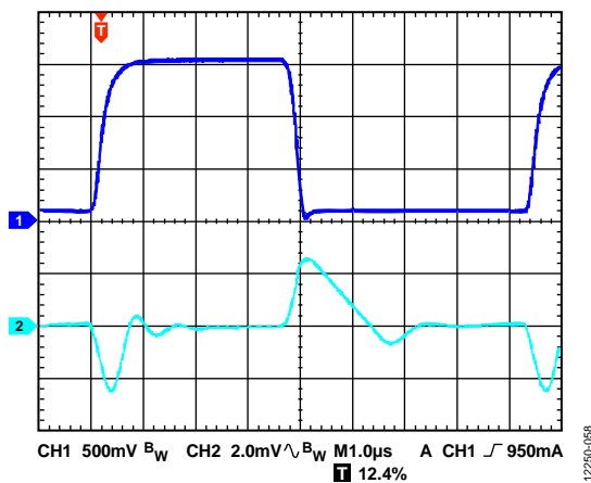
Figure 58. Output Transient Response, V_{\text{OUT}} = 5\text{ V} , C_{\text{OUT}} = 4.7\ \mu\text{F}
