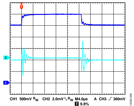
Figure 55. Line Transient Response, 2.5 V to 3 V, I_{LOAD} = 2\text{ A} , Adjustable Version, V_{OUT} = 1.2\text{ V} , CH1 = V_{IN} , CH2 = V_{OUT}
