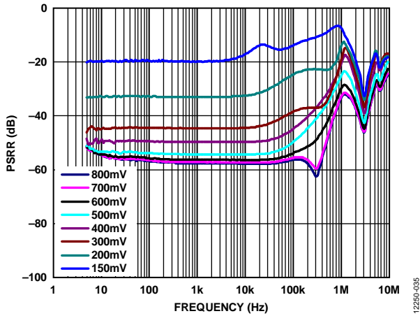
Figure 35. Power Supply Rejection Ratio (PSRR) vs. Frequency, V_{OUT} = 5 V , 2 A Load Current, Various Headroom Voltages
