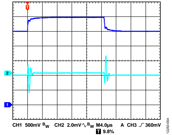
Figure 54. Line Transient Response, 2.5 V to 3 V, I_{LOAD} = 500\text{ mA} , Adjustable Version, V_{OUT} = 1.2\text{ V} , CH1 = V_{IN} , CH2 = V_{OUT}
