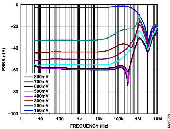
Figure 30. Power Supply Rejection Ratio (PSRR) vs. Frequency, V_{OUT} = 3 V , 2 A Load Current, Various Headroom Voltages
