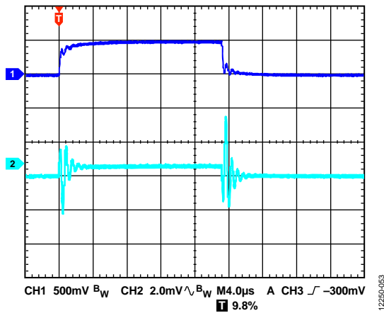
Figure 53. Line Transient Response, 6 V to 6.5 V, I_{LOAD} = 2\text{ A} , V_{OUT} = 5\text{ V} , CH1 = V_{IN} , CH2 = V_{OUT}
