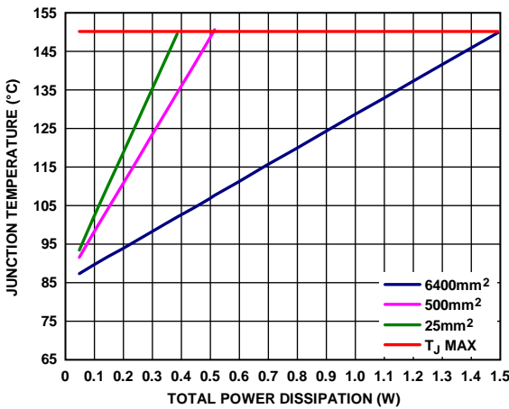
Figure 67. LFCSP, T_A = 85^\circ\text{C}
