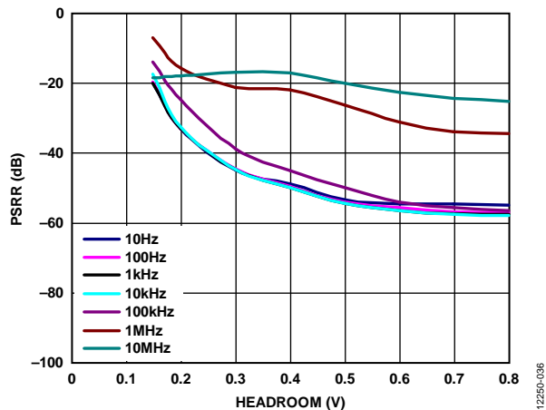
Figure 36. Power Supply Rejection Ratio (PSRR) vs. Headroom, V_{OUT} = 5 V , 2 A Load Current, Different Frequencies
