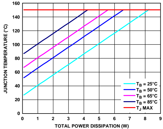
Figure 68. LFCSP Power Dissipation for Various Board Temperatures
