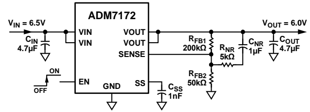
Figure 64. Noise Reduction Modification
