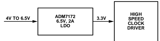
Figure 69. Clock Driver Power
