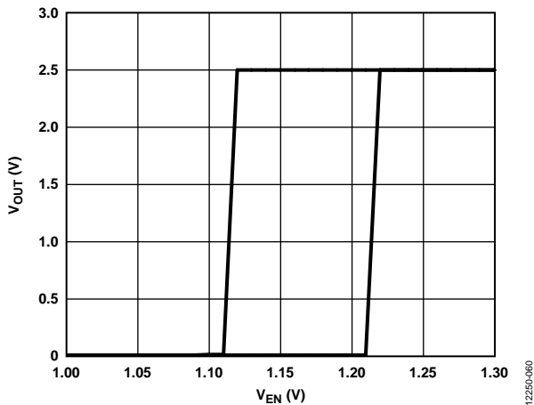
Figure 60. Typical V OUT Response to EN Pin Operation
