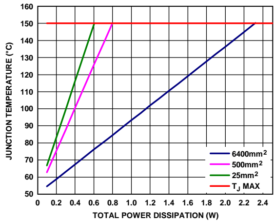
Figure 66. LFCSP, T_A = 50^\circ\text{C}
