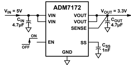
Figure 1. ADM7172 with Fixed Output Voltage, 3.3 V
