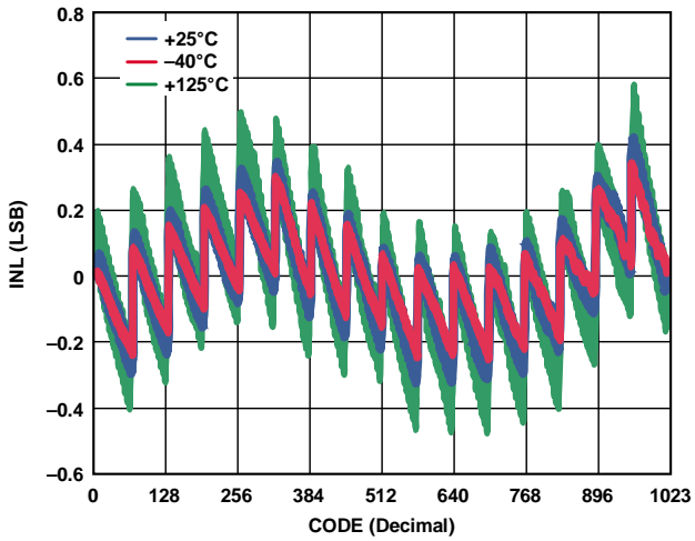
Figure 7. R-INL vs. Code vs. Temperature
