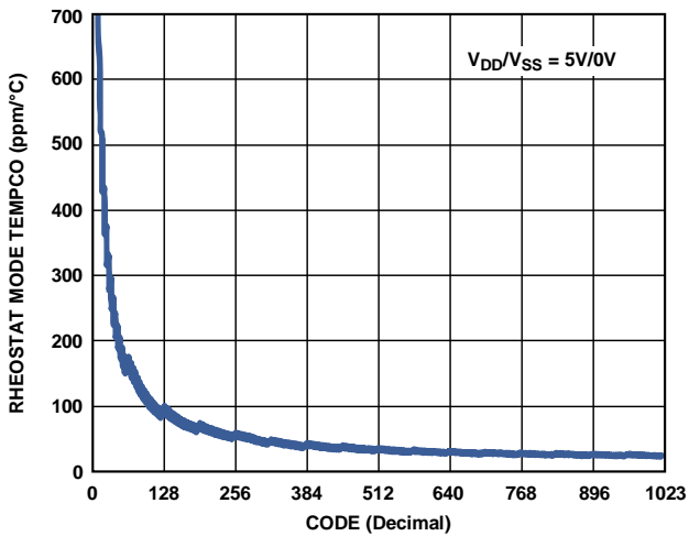
Figure 9. Tempco \Delta R_{WW}/\Delta T vs. Code
