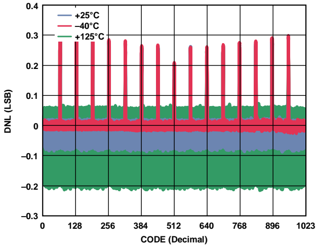
Figure 8. R-DNL vs. Code vs. Temperature
