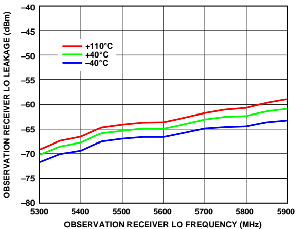
Figure 219. Observation Receiver LO Leakage vs. Observation Receiver LO Frequency, 0 dB Receiver Attenuation, 200 MHz RF Bandwidth, 245.76 MSPS Sample Rate
