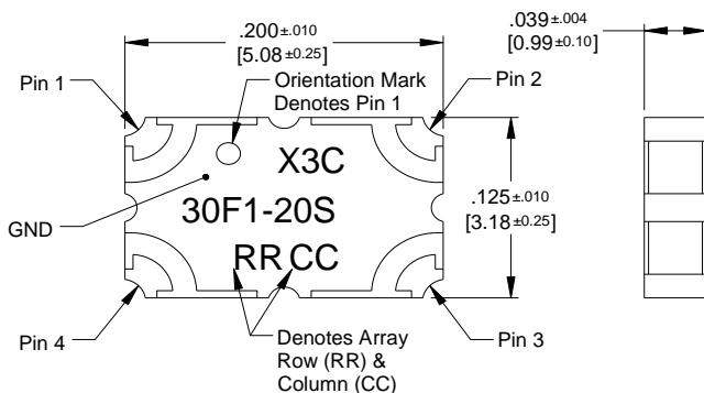
Dimensions are in Inches [Millimeters] X3C30F1-20S Mechanical Outline
