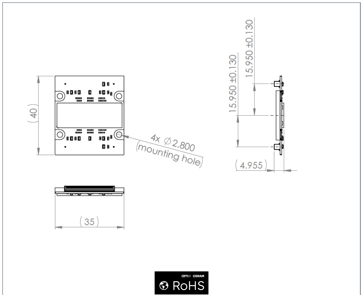
Figure 33: DR2K7 / DR2x2K7 / DR4K3.5 Invar package outline drawing
