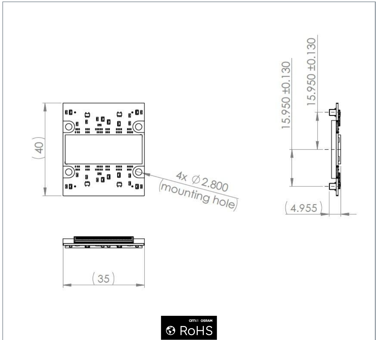
Figure 38: DR2x4K7 / DR8K3.5 Invar package outline drawing
