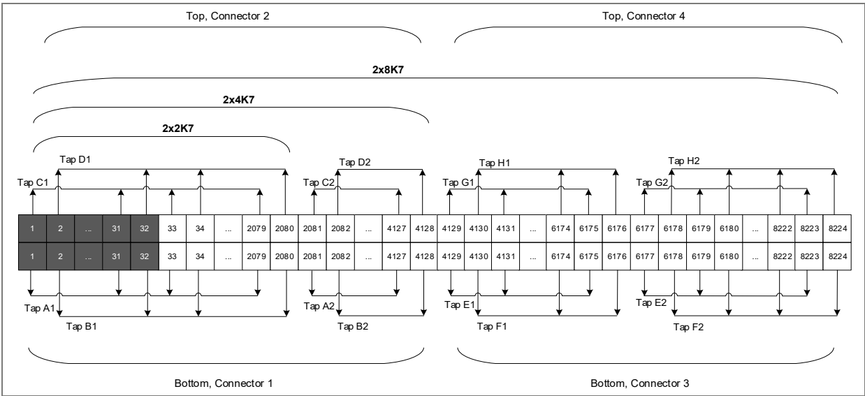
Figure 20: Tap organization DR2x2K7, DR2x4K7, DR2x8K7
