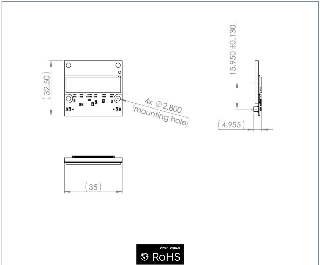
Figure 37: DR4K7 Invar package outline drawing
