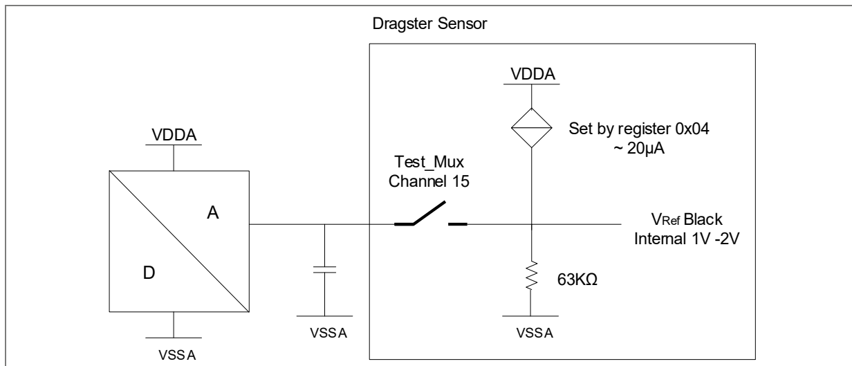
Figure 31: Equivalent load scheme for use of external DAC
