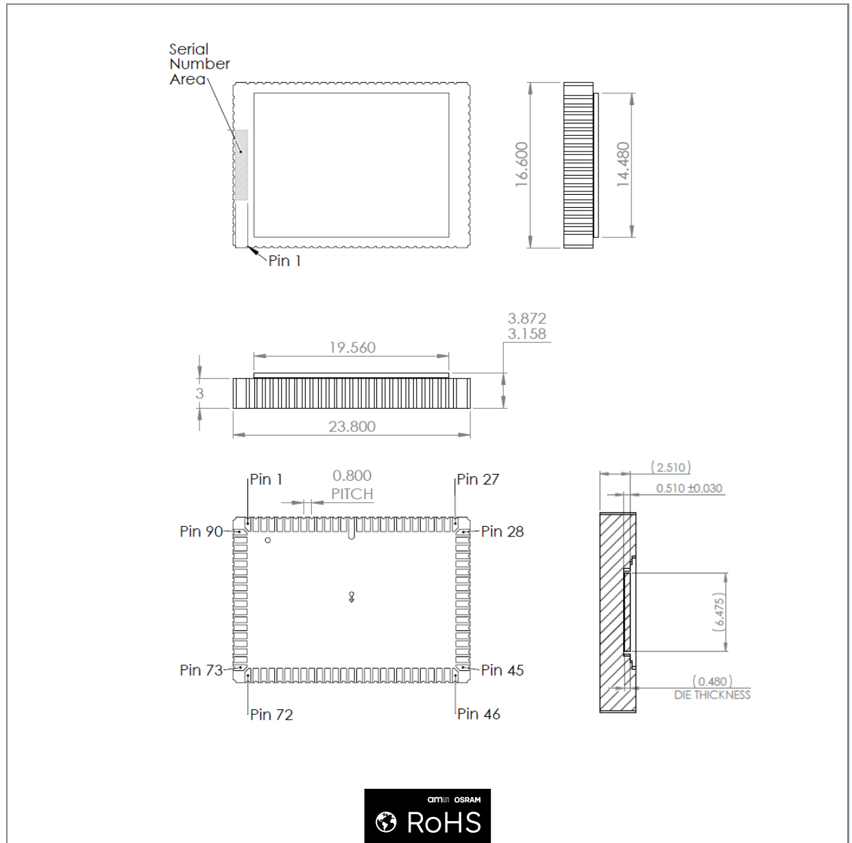
Figure 36: DR4K3.5 LCC ceramic package outline drawing
