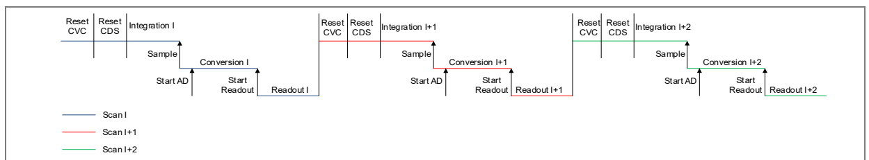
Figure 25: Dragster sequential timings
