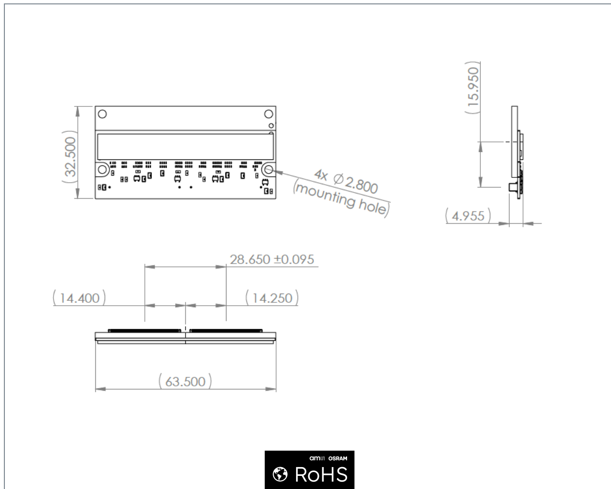
Figure 40: DR8K7 Invar package outline drawing
