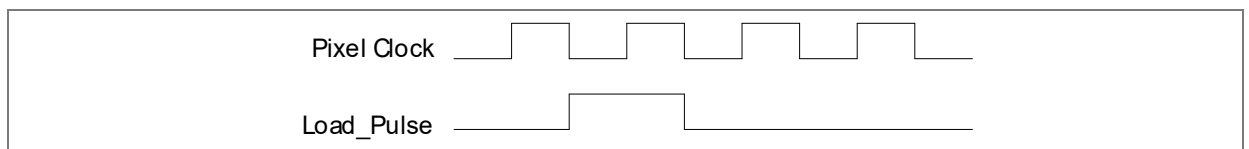
Figure 24: LOAD_PULSE signal generated with correct timing (1)
