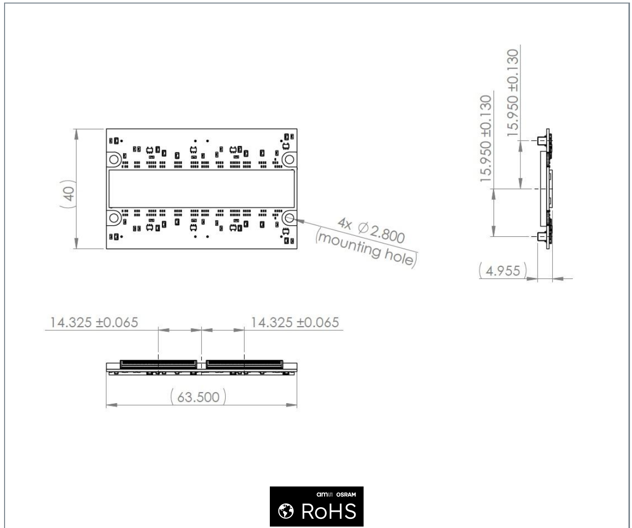
Figure 41: DR2x8K7 / DR16K3.5 Invar package outline drawing
