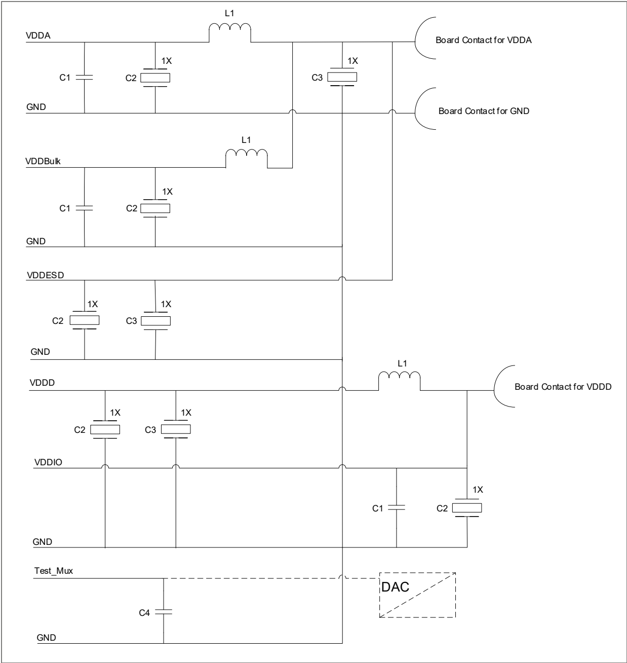
Figure 29: Recommended power supply strategy for the sensor headboard
