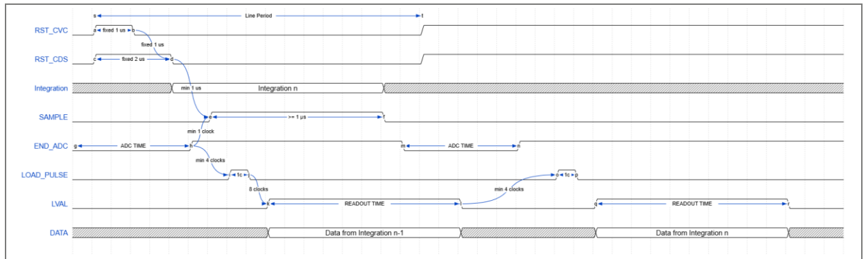
Figure 26: Timing diagram – end of readout entering idle
