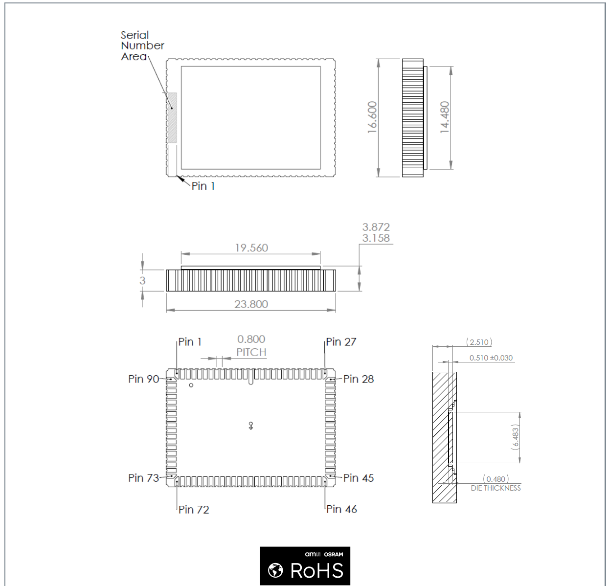
Figure 35: DR2x2K7 LCC ceramic package outline drawing
