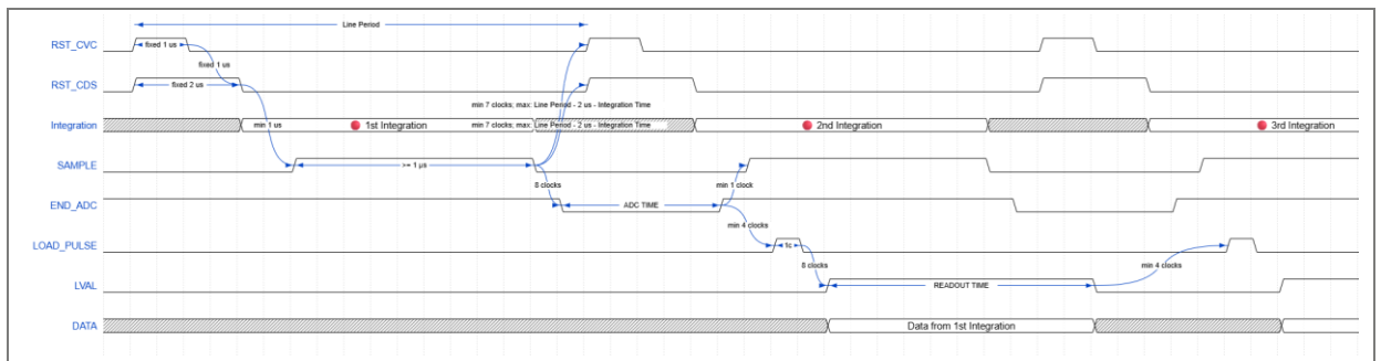
Figure 23: Dragster interleaved integration timing, for a fixed line period
