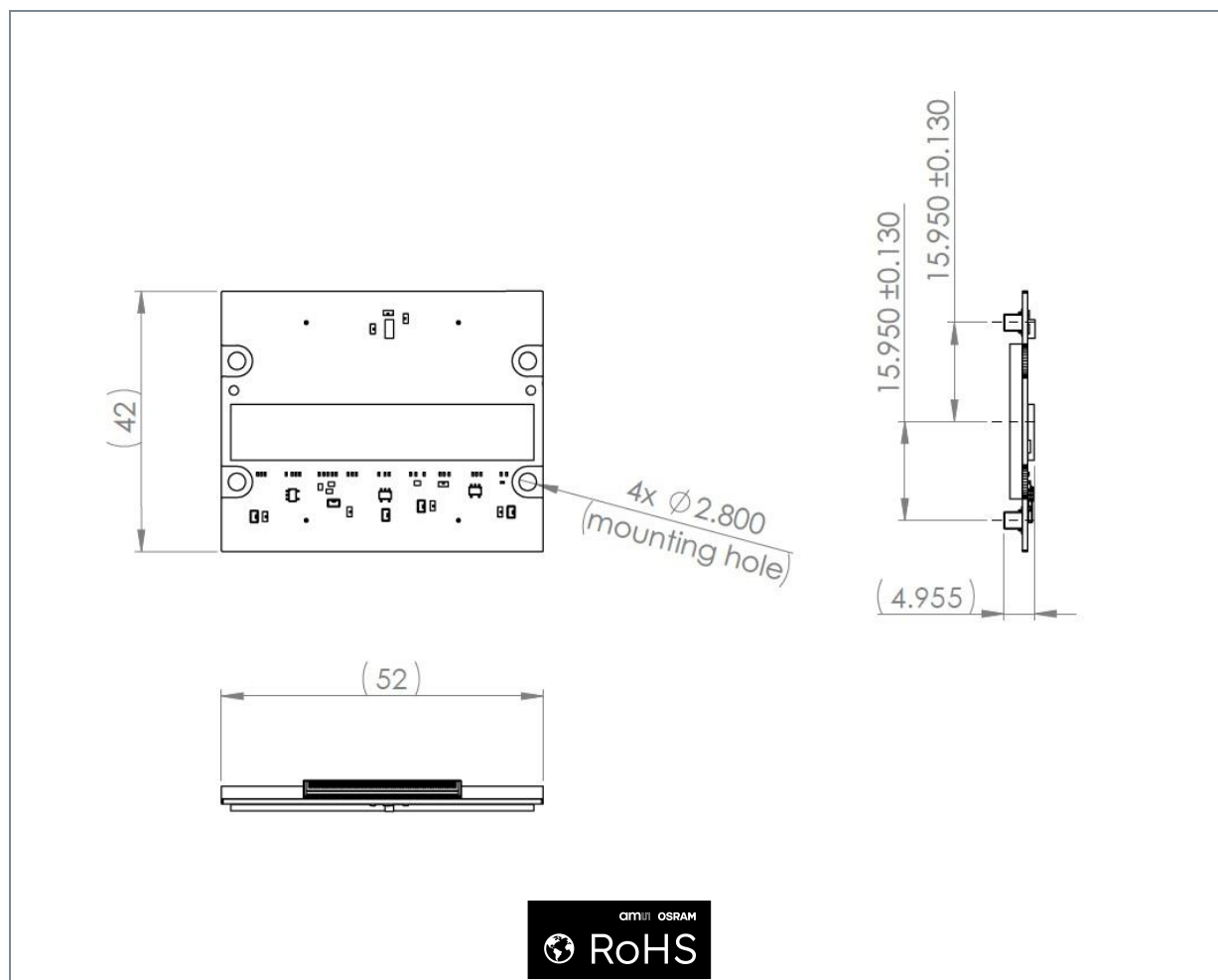
Figure 39: DR6K7 Invar package outline drawing
