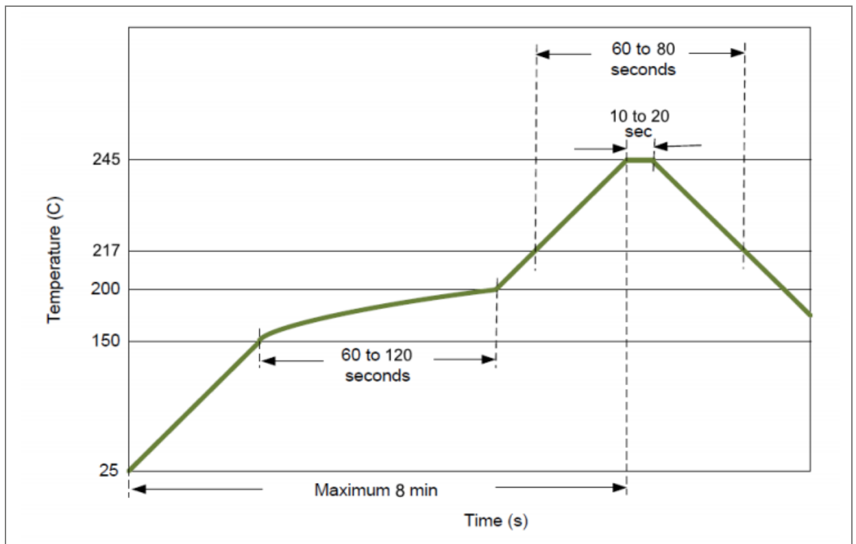
Figure 32: Solder reflow profile graph
