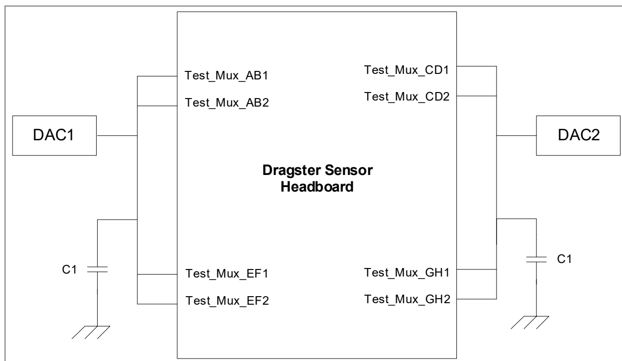
Figure 30: External components for the option to control the ADC offset by an external DAC for the case of a sensor with four segments
