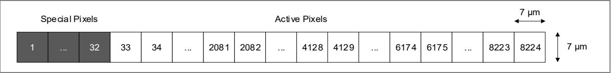
Figure 7: Placement of pixels sensors with 7 \mu\text{m} pixel pitch (DR8K7)
