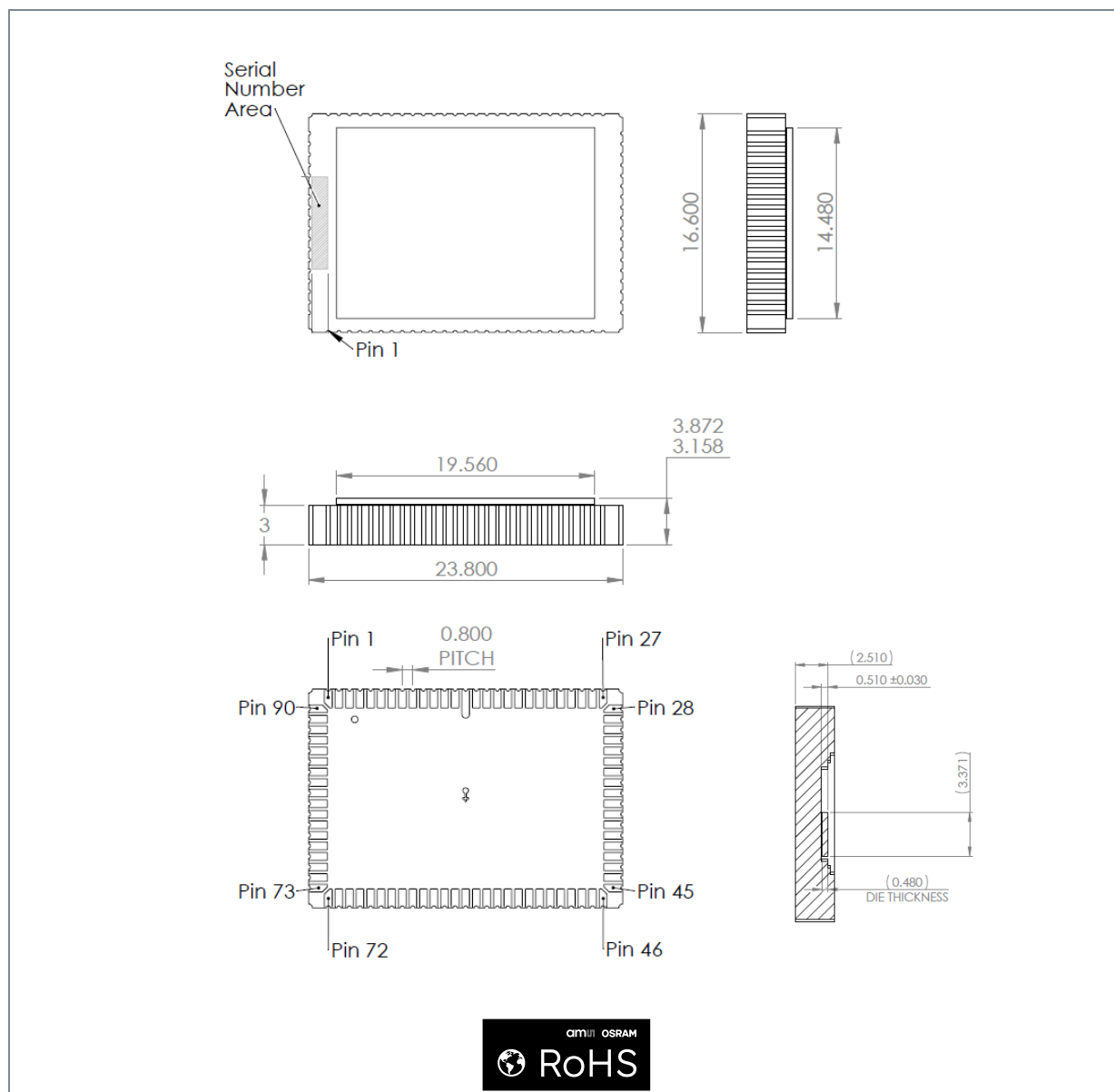
Figure 34: DR2K7 LCC ceramic package outline drawing
