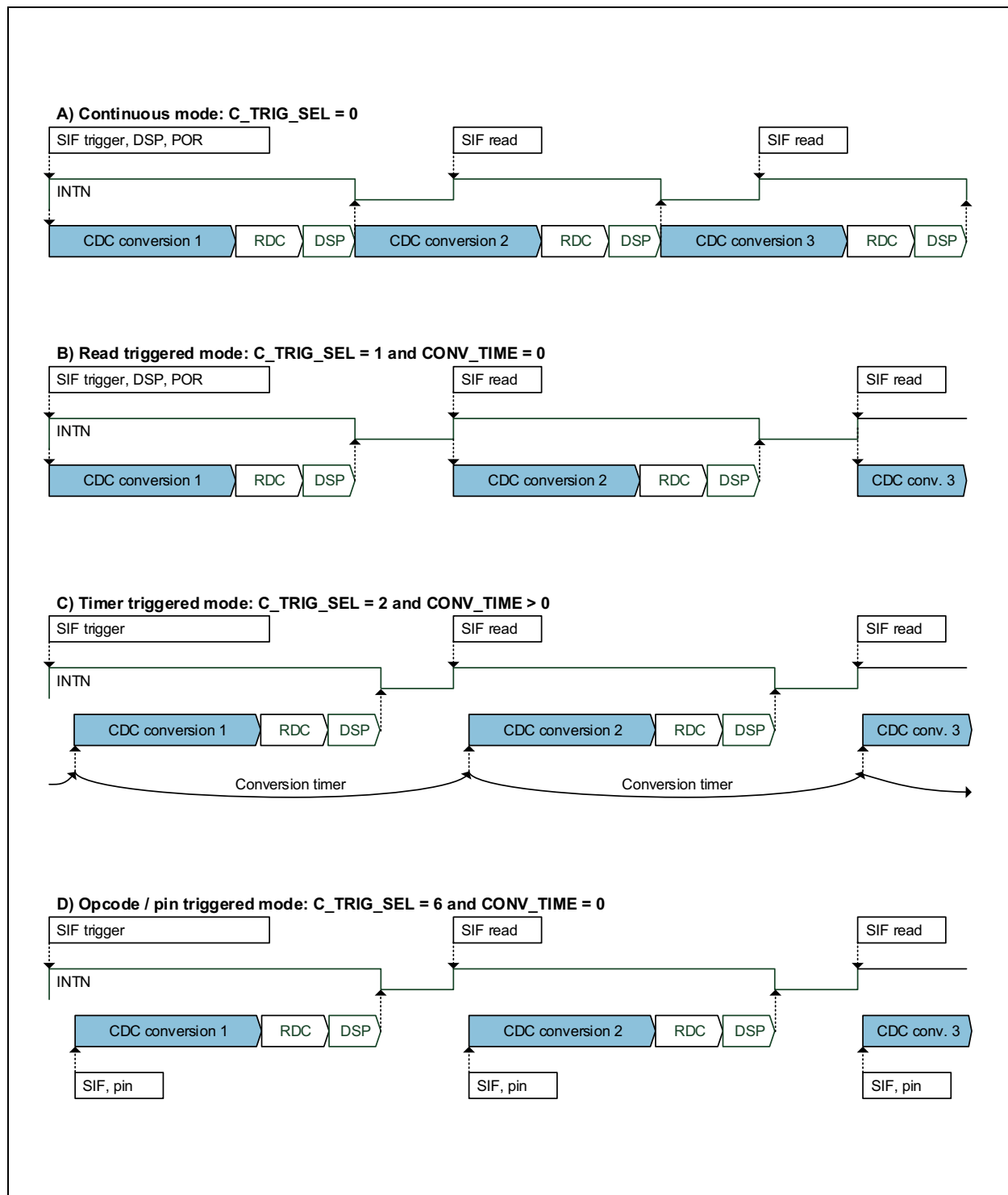
Figure 78: Conversion Modes
