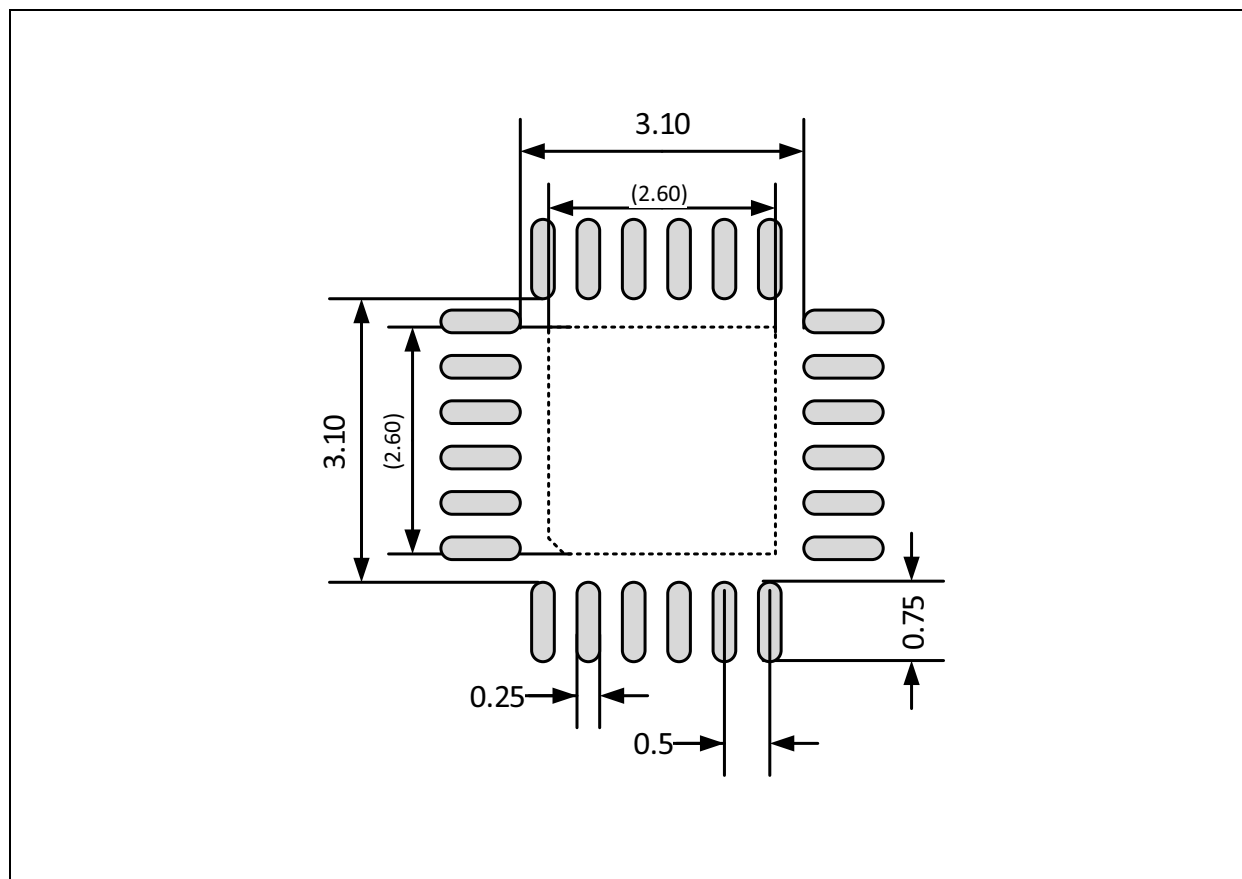
Figure 140: Landing Pattern
