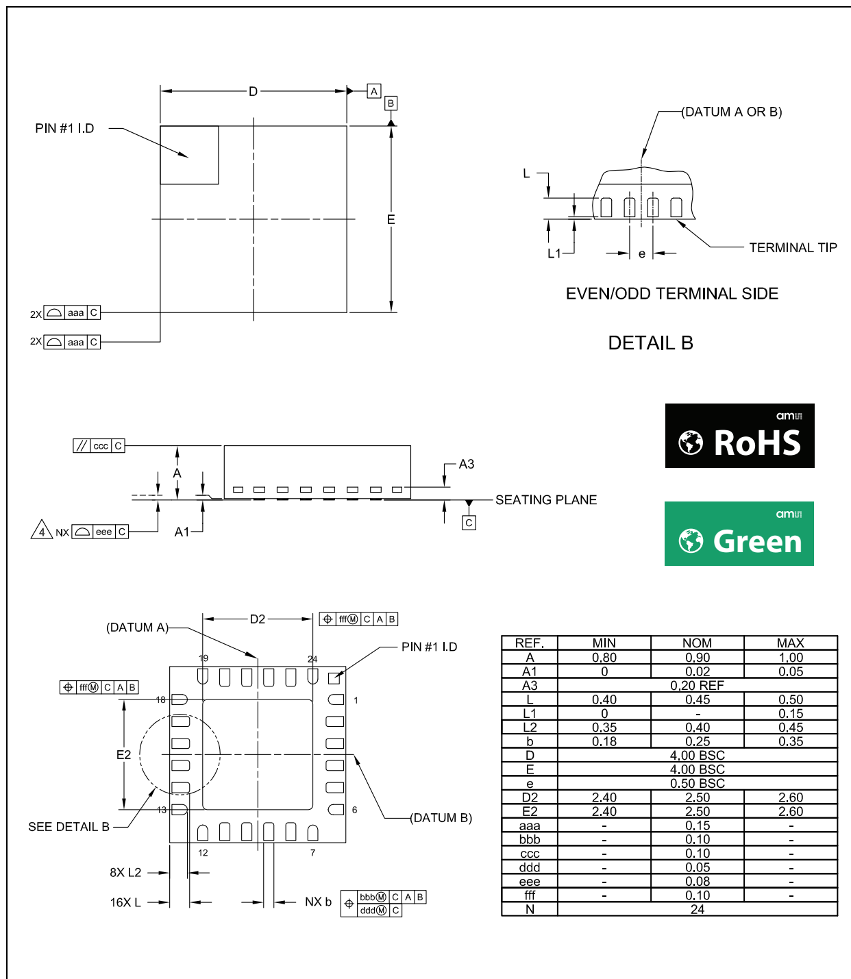
Figure 137: Package Drawing (QFN24)
