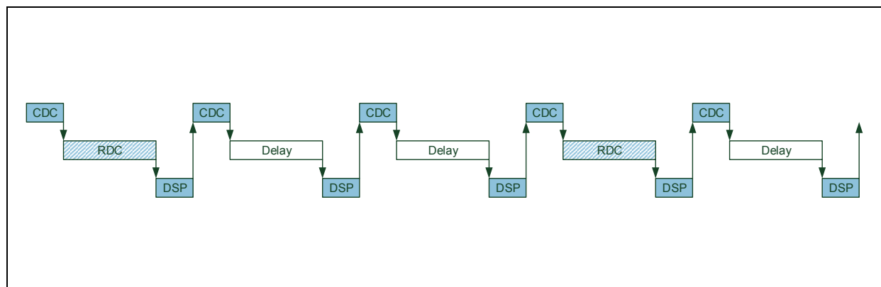
Figure 96: RDC Timing, Triggered by DSP in Synchronous Mode
