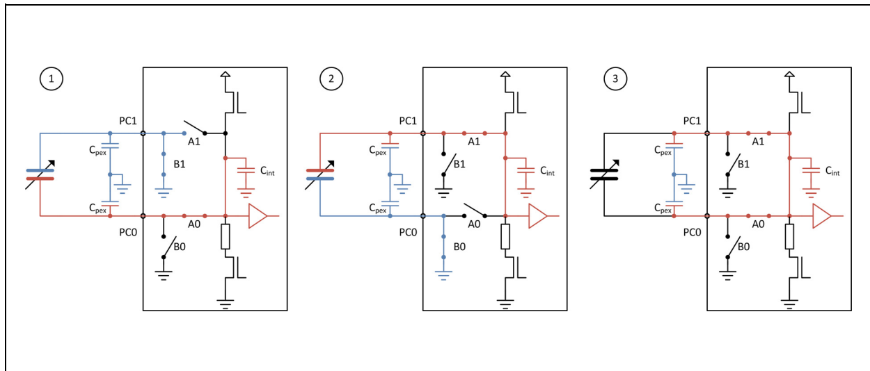
Figure 81: External Compensation
