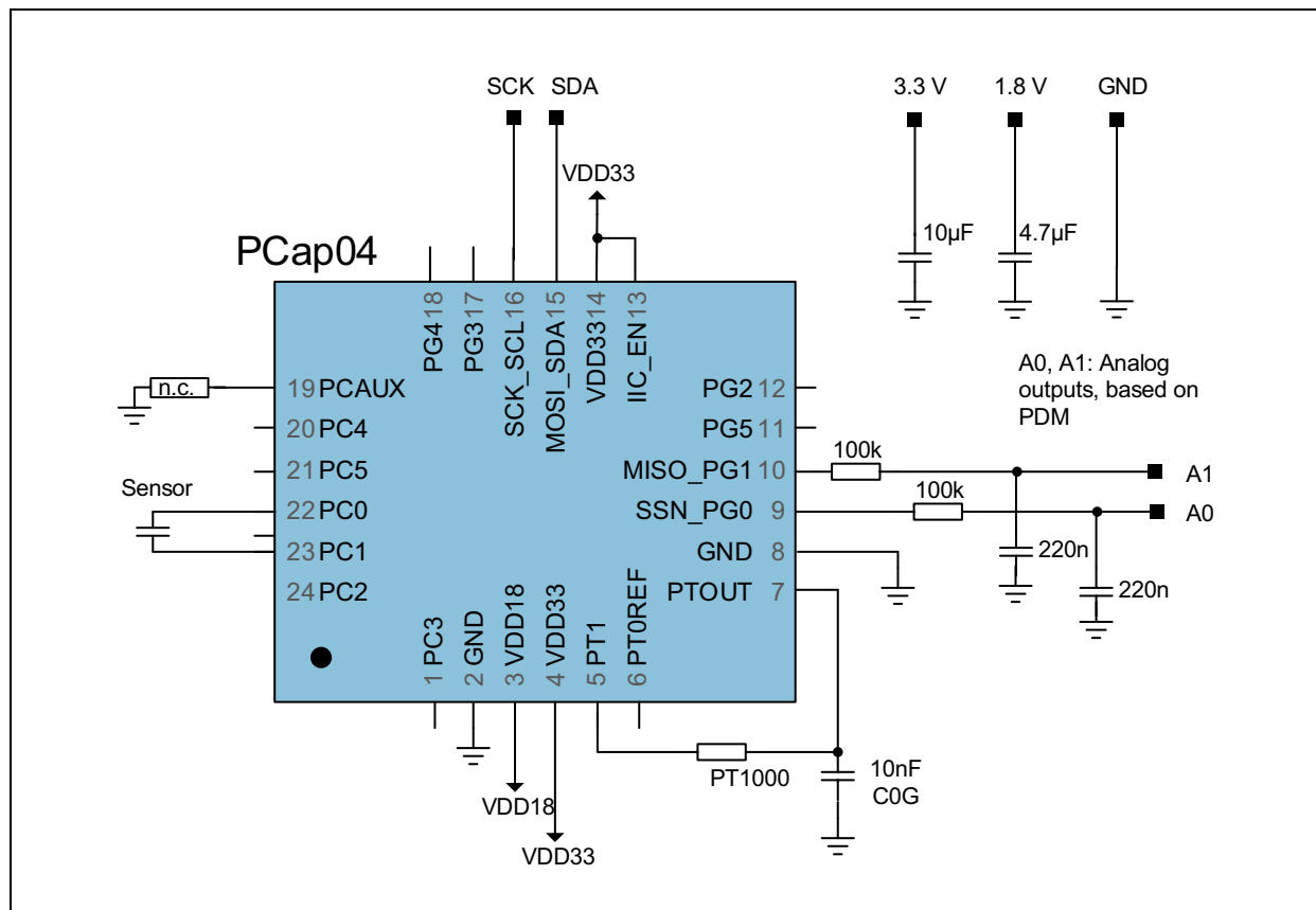
Figure 135: Typical Schematics with I 2 C Interface and PDM Analog Outputs
