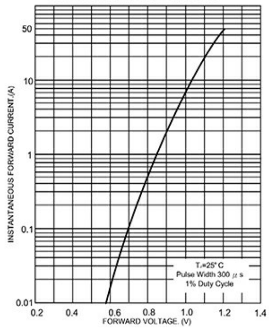
FIG.2 - TYPICAL FORWARD CHARACTERISTICS
