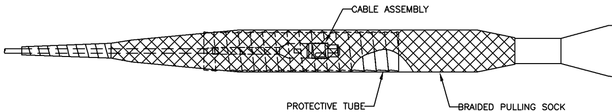
PULLING SOCK TOP END
