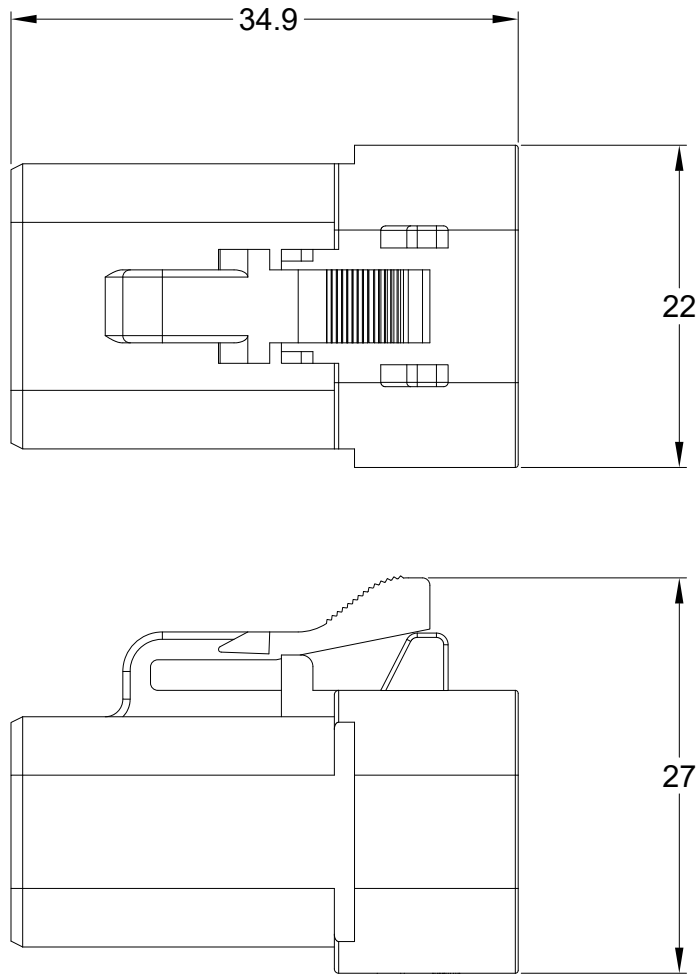
REFERENCE DIMENSIONS - ASSEMBLED
