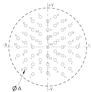
53 Contacts Size 20
