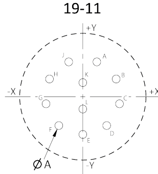
11 Contacts Size 16
