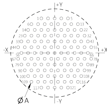
121 Contacts Size 23
