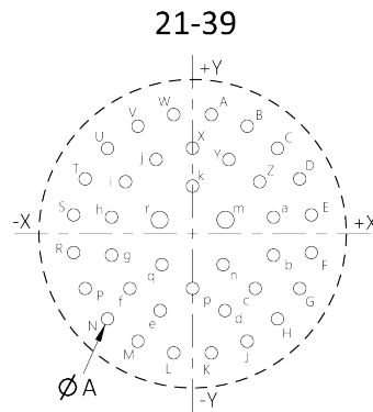
37 Contacts Size 20 2 Contacts Size 16
