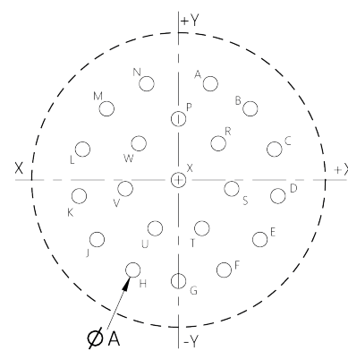
21 Contacts Size 16
