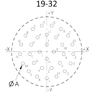
32 Contacts Size 20
