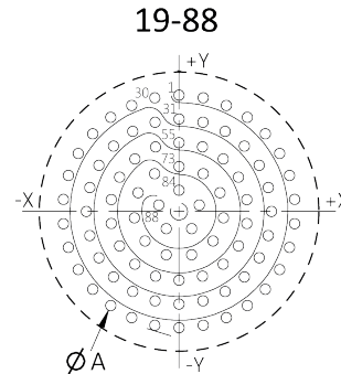
88 Contacts Size 23
