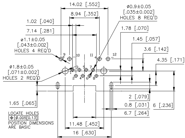
RECOMMENDED P.C.B LAYOUT (COMPONENT SIDE OF BOARD TOLERANCES: +/- .05[.002])
