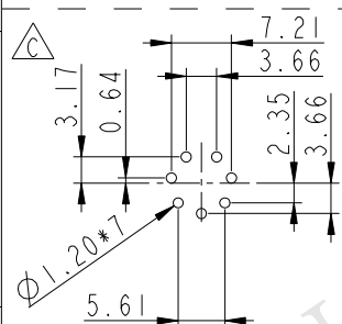
7 Pin Male Connector Male Pin PCB Layout
