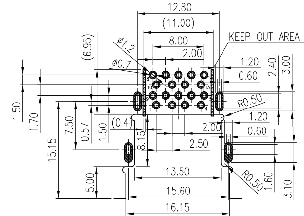
RECOMMENDED P.C.B LAYOUT TOLERANCE: \pm 0.05 (TOP VIEWS)
