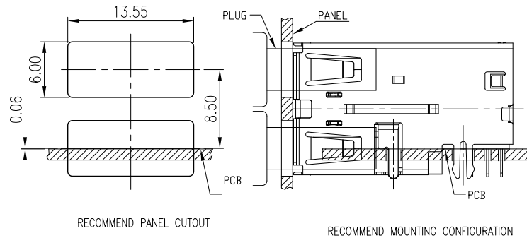
RECOMMEND MOUNTING CONFIGURATION
