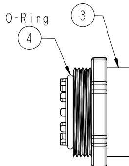
Extension Nut
