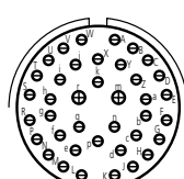
SIZE 21 SHELL
