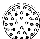
SIZE 19 SHELL
