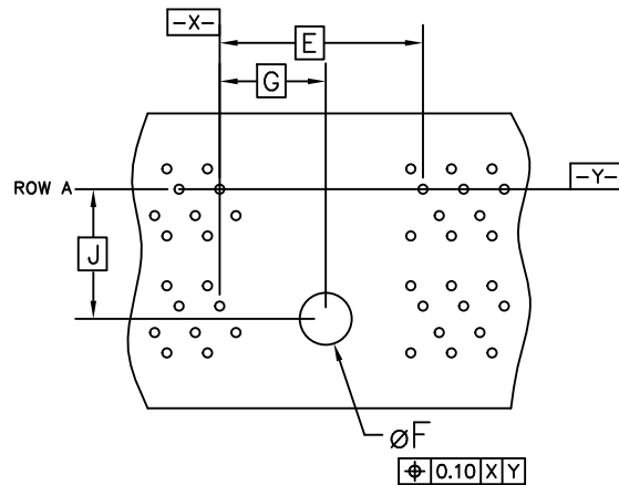
eHSD 5 ROW BACKPLANE HOLE PATTERN, CONNECTOR SIDE GUIDE PIN
