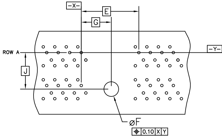
eHSD 5+ ROW BACKPLANE HOLE PATTERN, CONNECTOR SIDE GUIDE PIN
