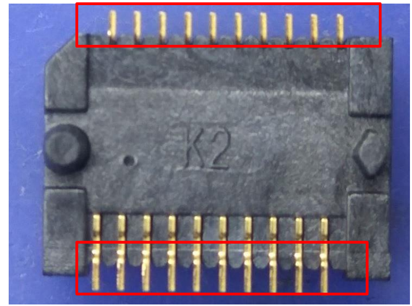
Plating gold flash on soldering pin area for new part number
