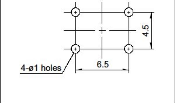
Viewed from mounting face.
