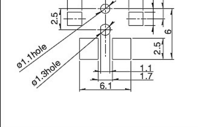
Viewed from direction A in the dimensions.
