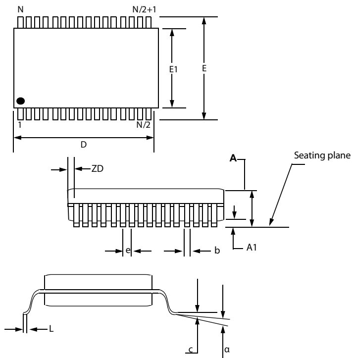
32-pin TSOP 2
