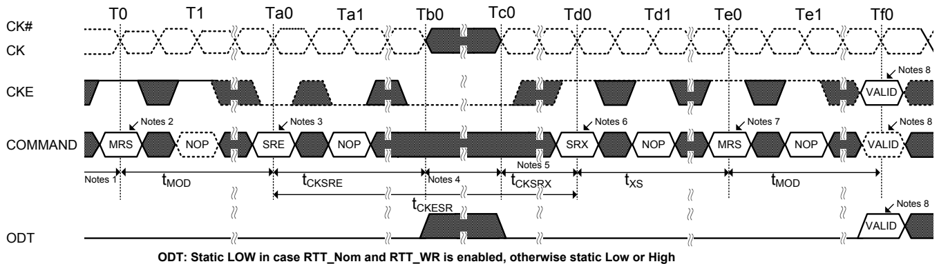
Figure 11. DLL-off mode READ Timing Operation
