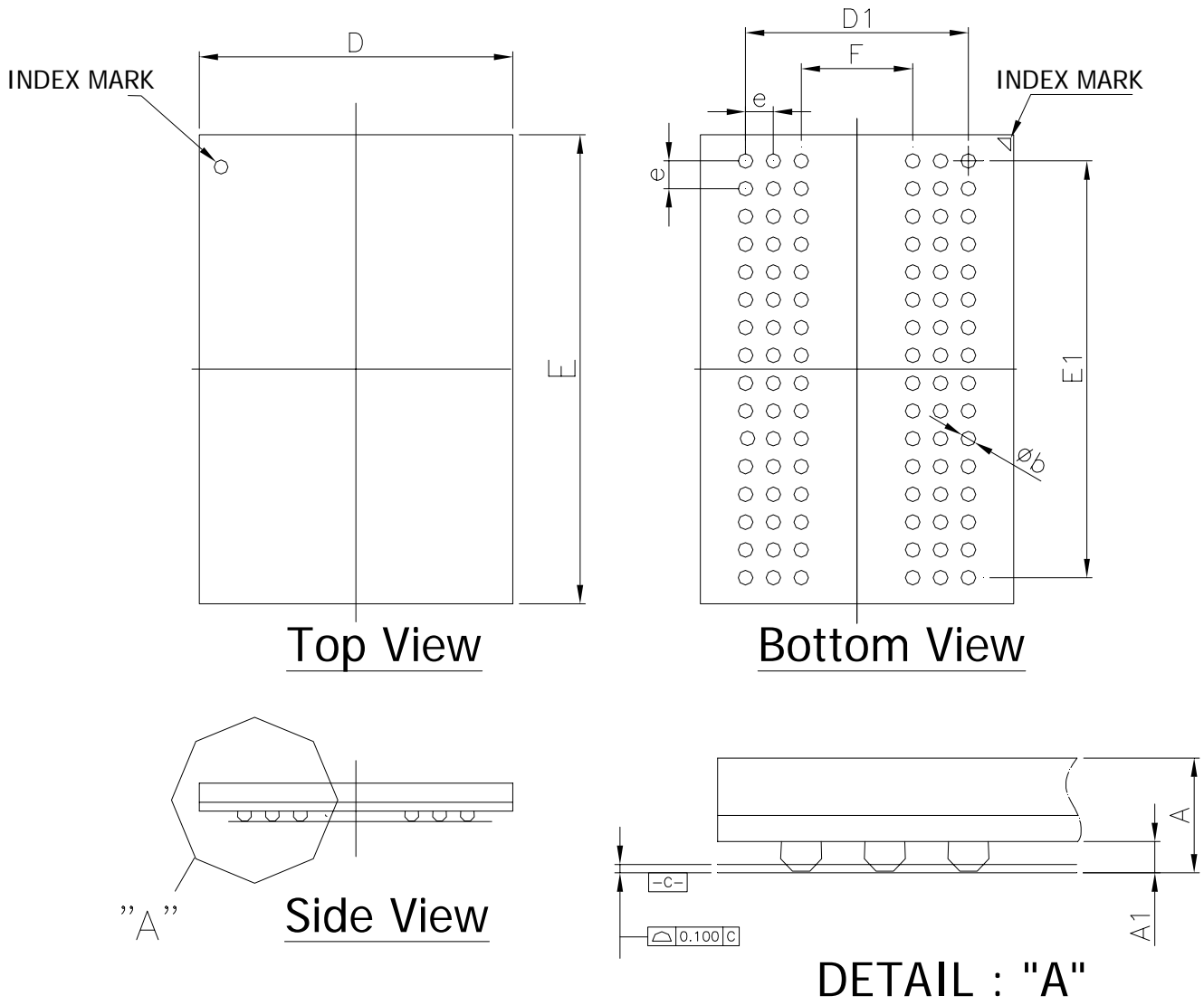
Figure 83. 96-Ball FBGA Package 9x13.5x1.2mm(max) Outline Drawing Information
