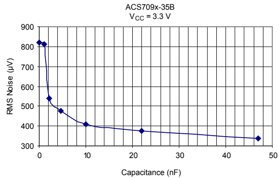
ACS709 Noise versus External Capacitor Value, C_F Capacitor connected between FILTER pin and GND
