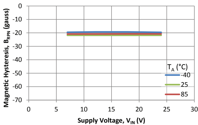
B RPN vs. V IN
