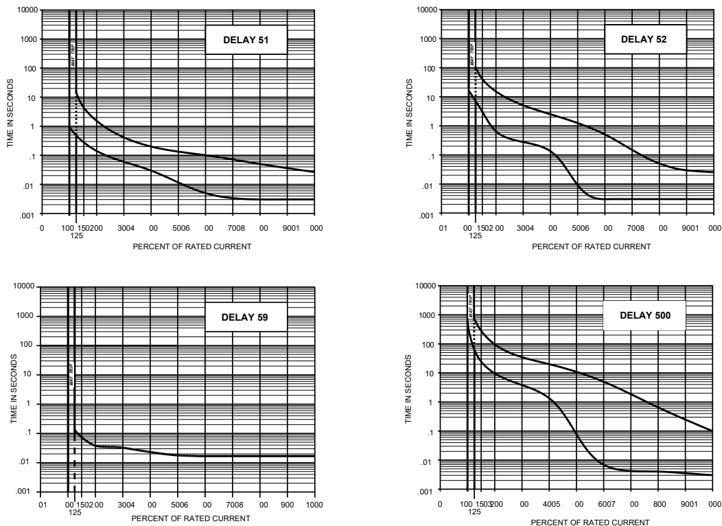
DC Delay Curves (typ)
