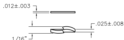
FLAT WASHER .215 O.D. x .120 I.D. SPLIT LOCKWASHER .212±.015 O.D. x .115 I.D.
