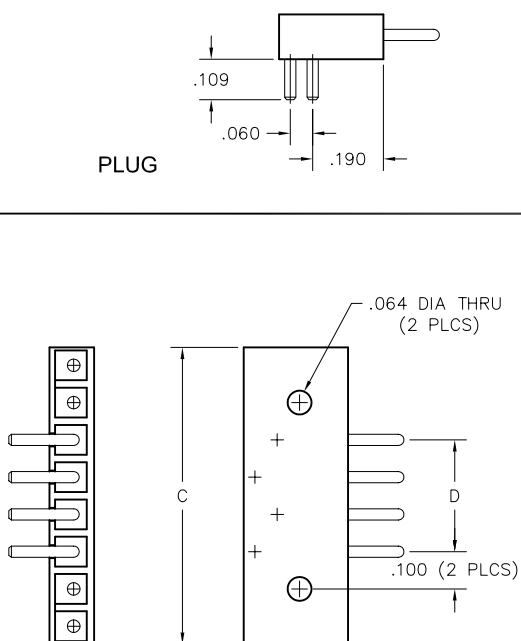
MOUNTING HOLES (OPTION: CD)
