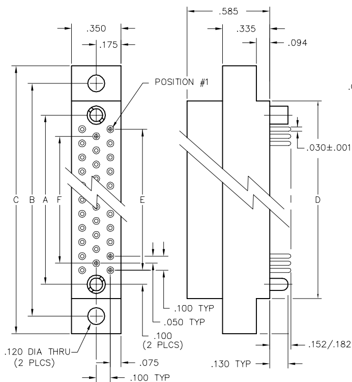
PLUG
