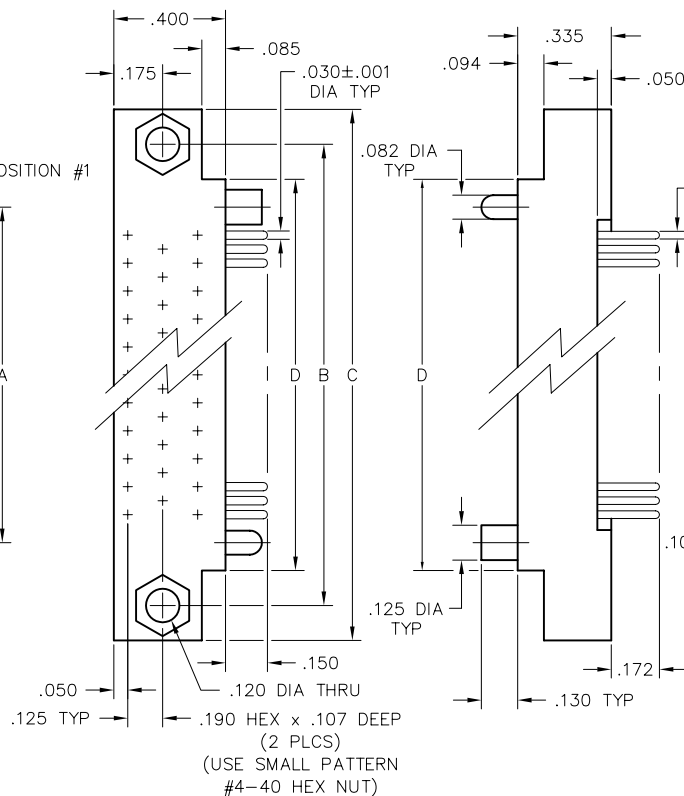
PLUG
