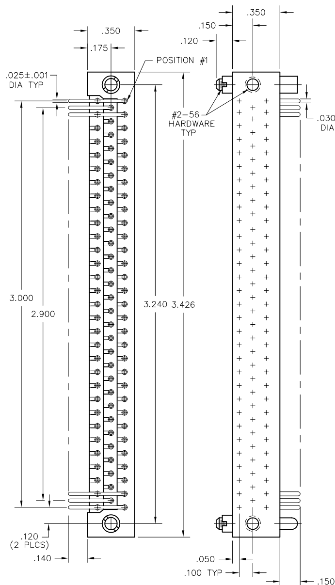
PLUG
