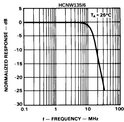
Figure 10. Frequency Response.
