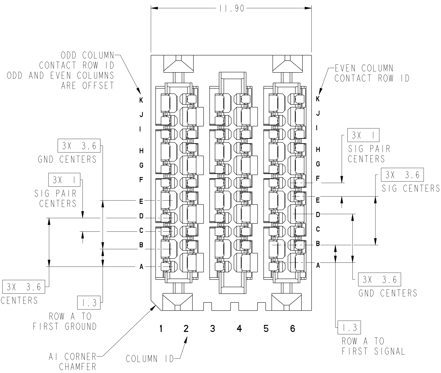
10137068-Y01LF (10137068-101LF STANDARD MATE CONNECTOR SHOWN) SCALE 7:1
