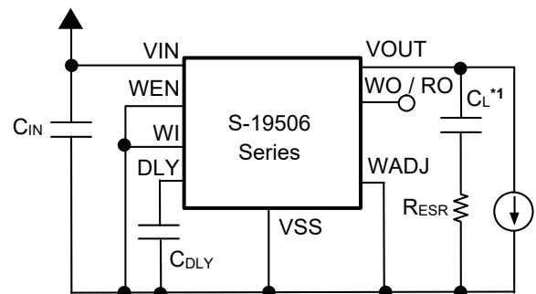
*1. C L : TDK Corporation CGA5L3X8R1H105K (1.0 μF) Figure 42
