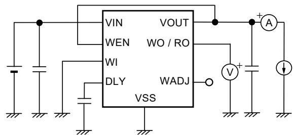
Figure 17 Test Circuit 6
