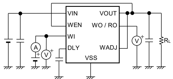
Figure 19 Test Circuit 8
