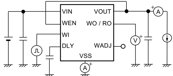
Figure 21 Test Circuit 10
