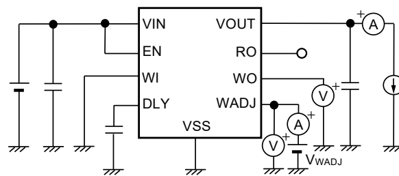
Figure 28 Test Circuit 8
