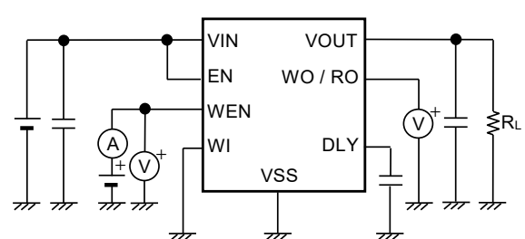
Figure 18 Test Circuit 8
