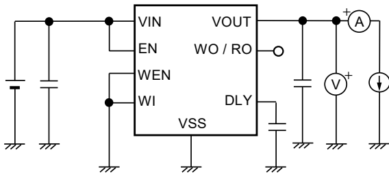
Figure 11 Test Circuit 1
