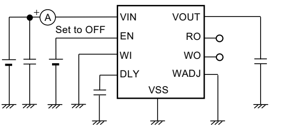
Figure 30 Test Circuit 10
