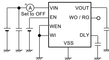
Figure 20 Test Circuit 10
