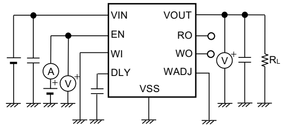
Figure 24 Test Circuit 4
