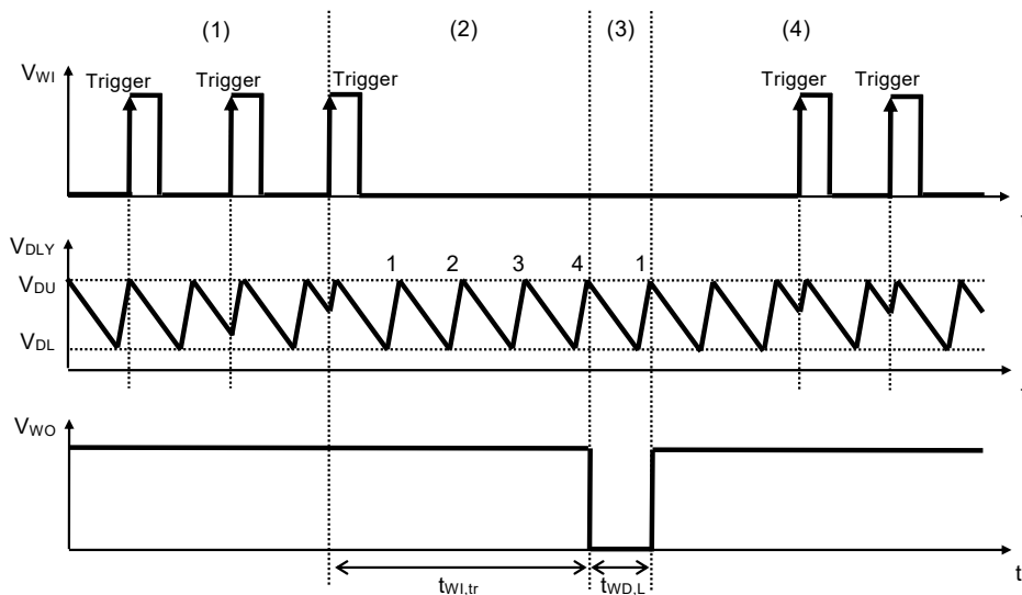
Figure 43 Timing Chart of Watchdog Timer Block
