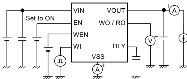
Figure 19 Test Circuit 9
