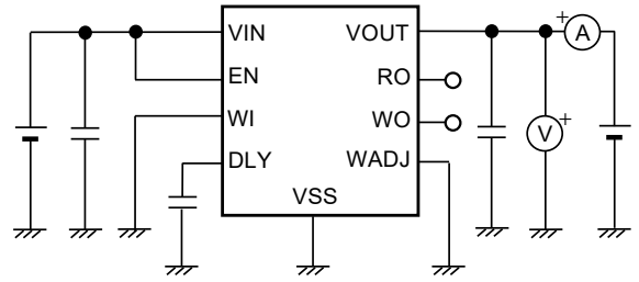
Figure 22 Test Circuit 2
