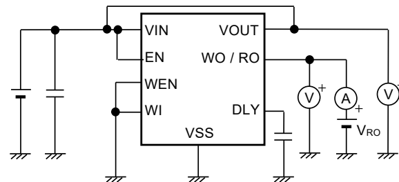
Figure 16 Test Circuit 6
