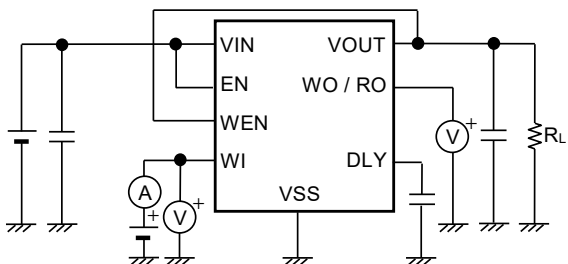
Figure 17 Test Circuit 7
