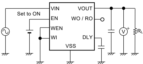
Figure 13 Test Circuit 3
