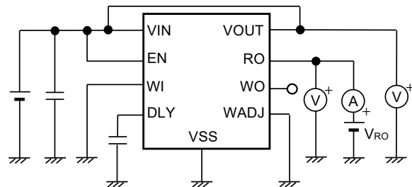
Figure 26 Test Circuit 6
