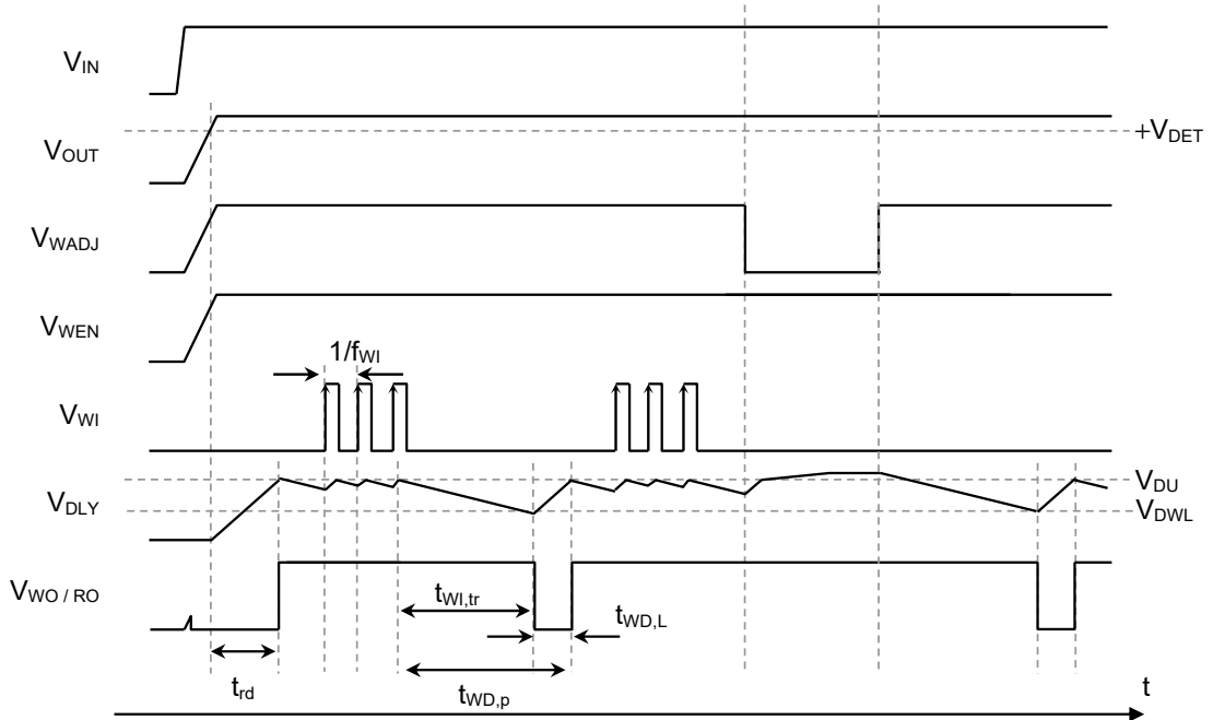
Figure 40 Example of Watchdog Timer Monitoring Operation 1
