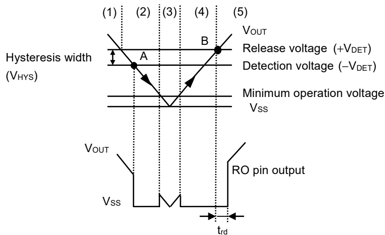
Figure 35 Timing Chart of Detector Block
