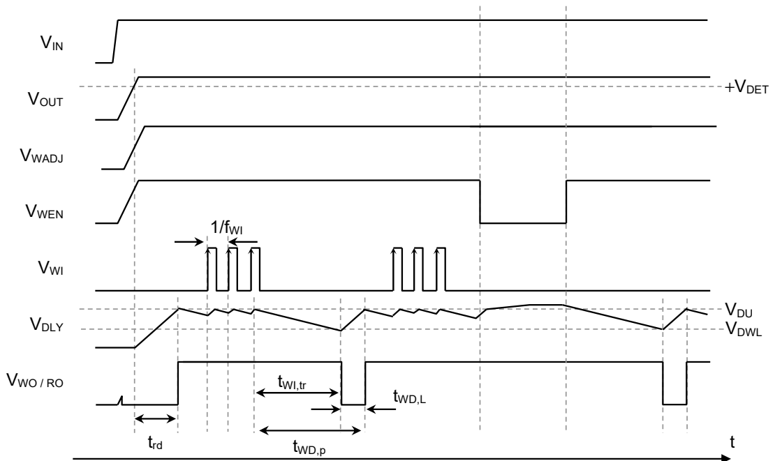
Figure 41 Example of Watchdog Timer Monitoring Operation 2
