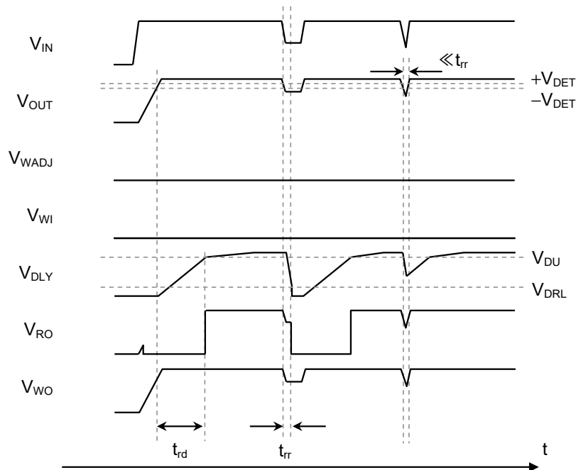
Figure 44 Example of Detector Operation
