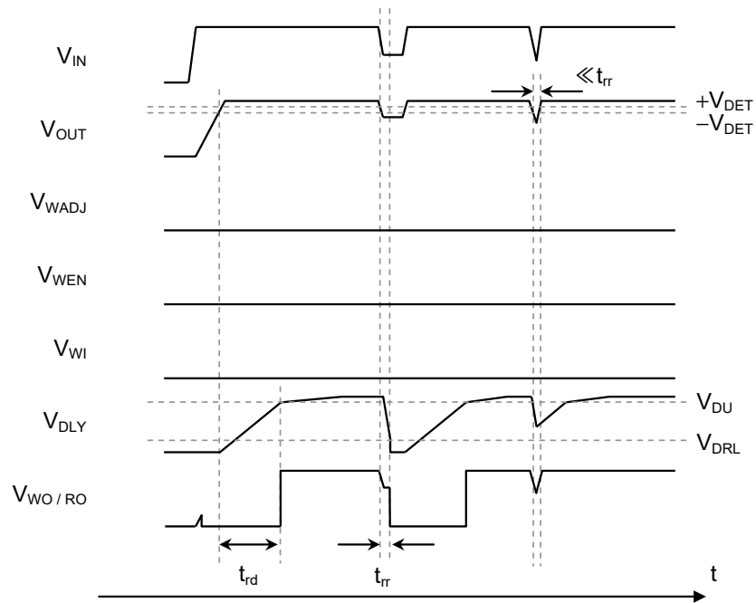
Figure 42 Example of Detector Operation
