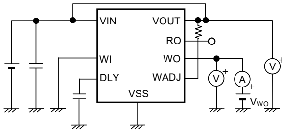
Figure 30 Test Circuit 11
