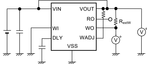
Figure 29 Test Circuit 10
