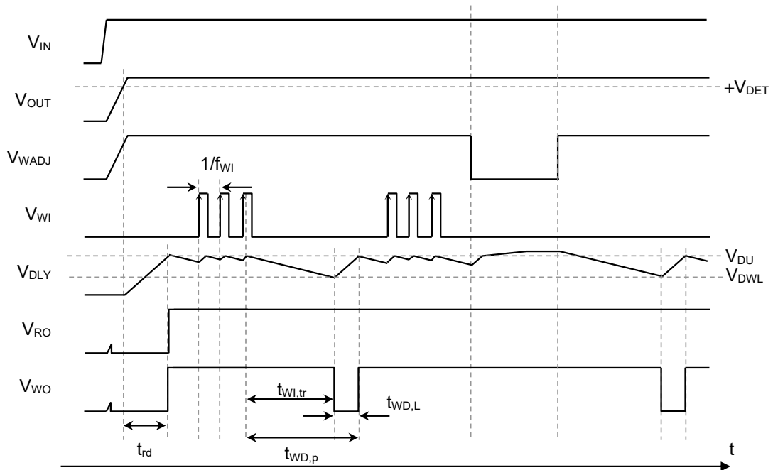
Figure 43 Example of Watchdog Timer Monitoring Operation
