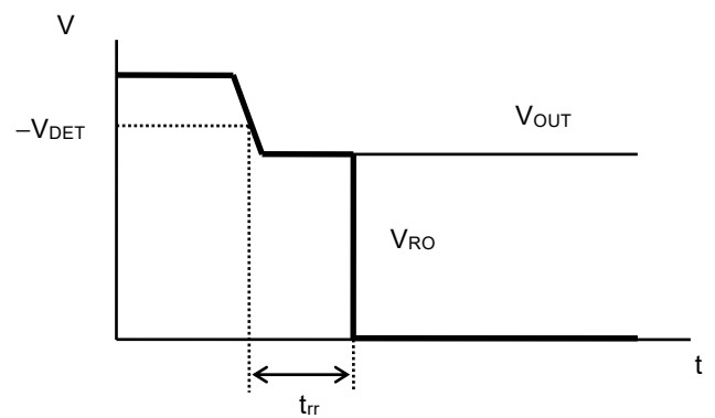
Figure 7 Reset Reaction Time
