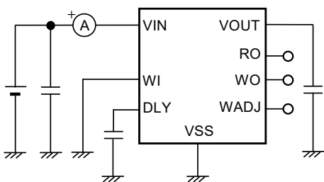
Figure 28 Test Circuit 9
