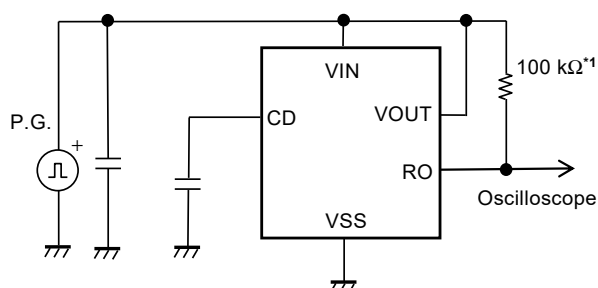
Figure 11 Test Circuit 5
