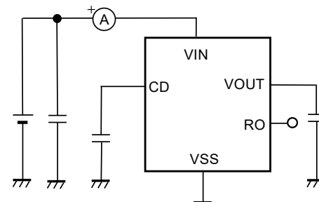
Figure 12 Test Circuit 6
