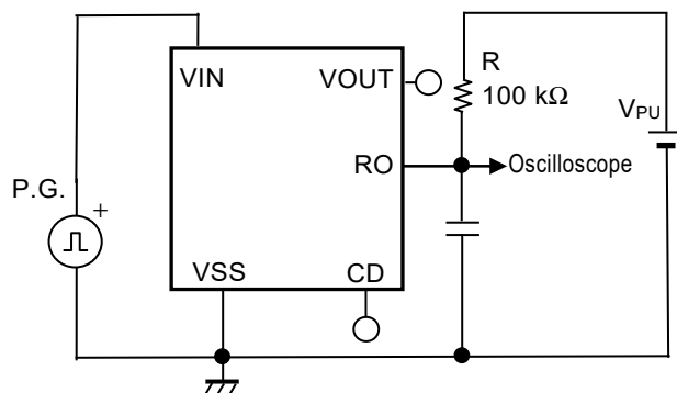
Figure 27 Test Circuit of Response Time
