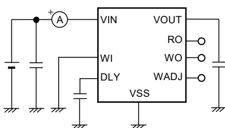
Figure 27 Test Circuit 9
