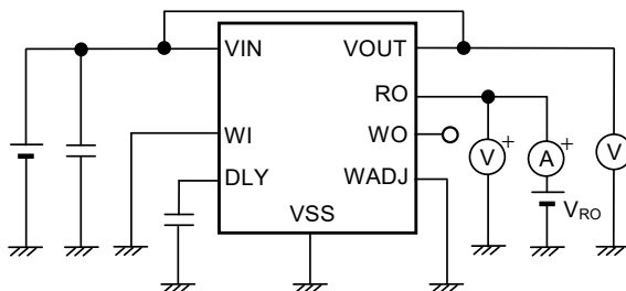
Figure 23 Test Circuit 5
