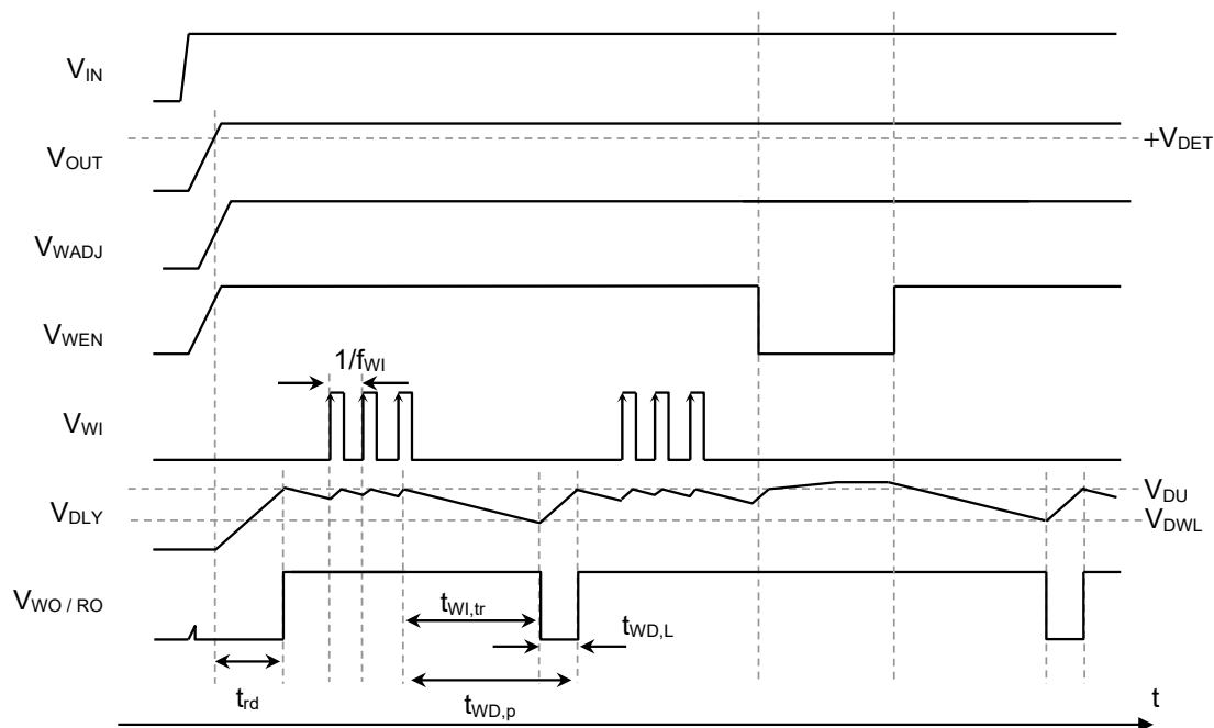
Figure 40 Example of Watchdog Timer Monitoring Operation 2
