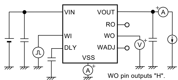
Figure 26 Test Circuit 8
