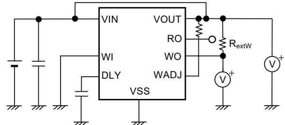
Figure 28 Test Circuit 10
