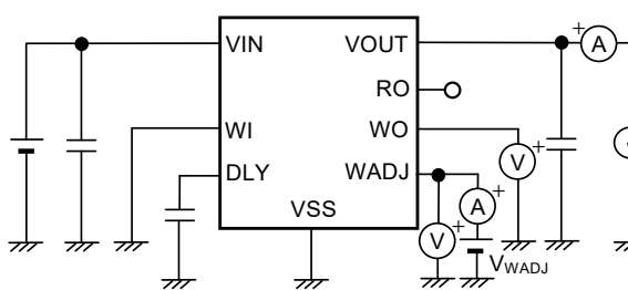
Figure 25 Test Circuit 7
