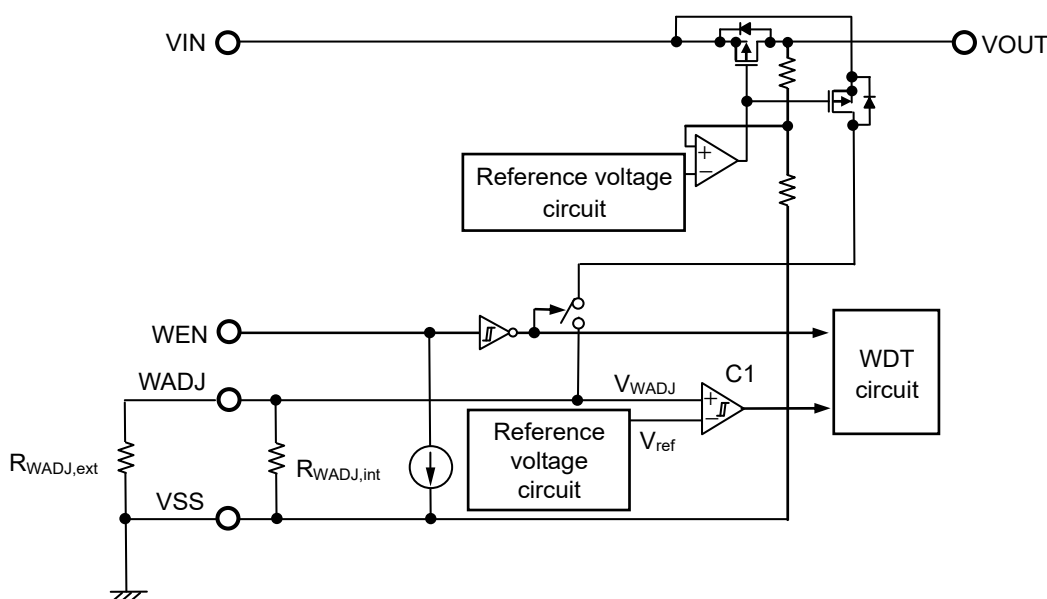
Figure 37 Operation of Output Current Detection Circuit
