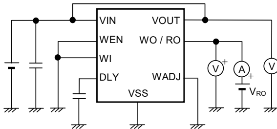
Figure 13 Test Circuit 5
