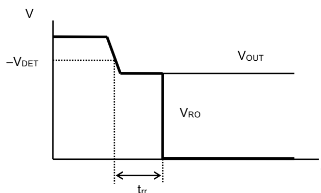
Figure 6 Reset Reaction Time
