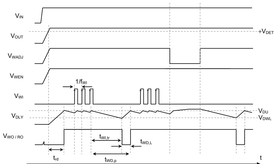
Figure 39 Example of Watchdog Timer Monitoring Operation 1
