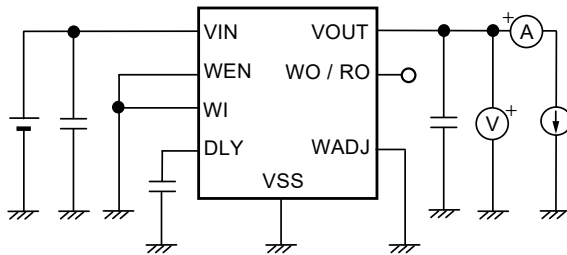
Figure 9 Test Circuit 1
