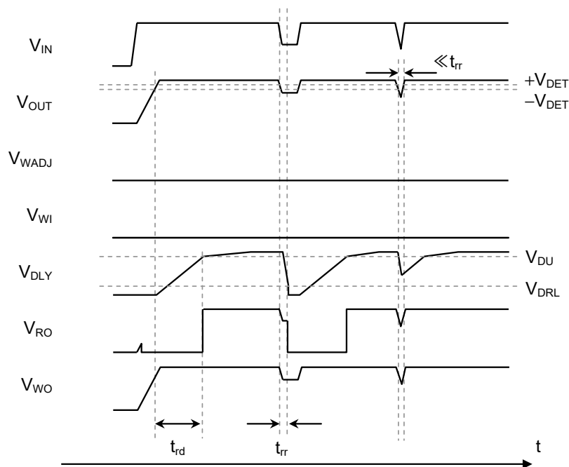
Figure 43 Example of Detector Operation
