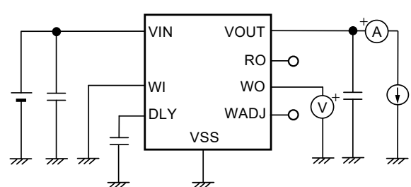
Figure 24 Test Circuit 6
