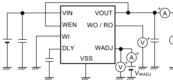
Figure 15 Test Circuit 7
