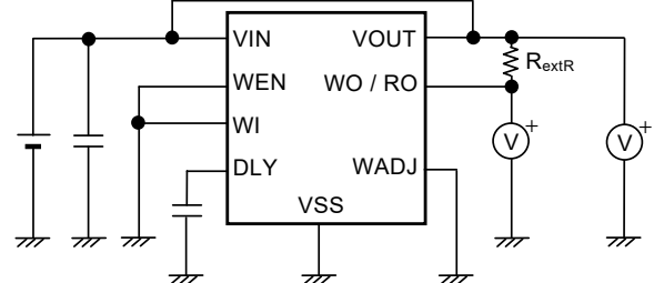
Figure 12 Test Circuit 4
