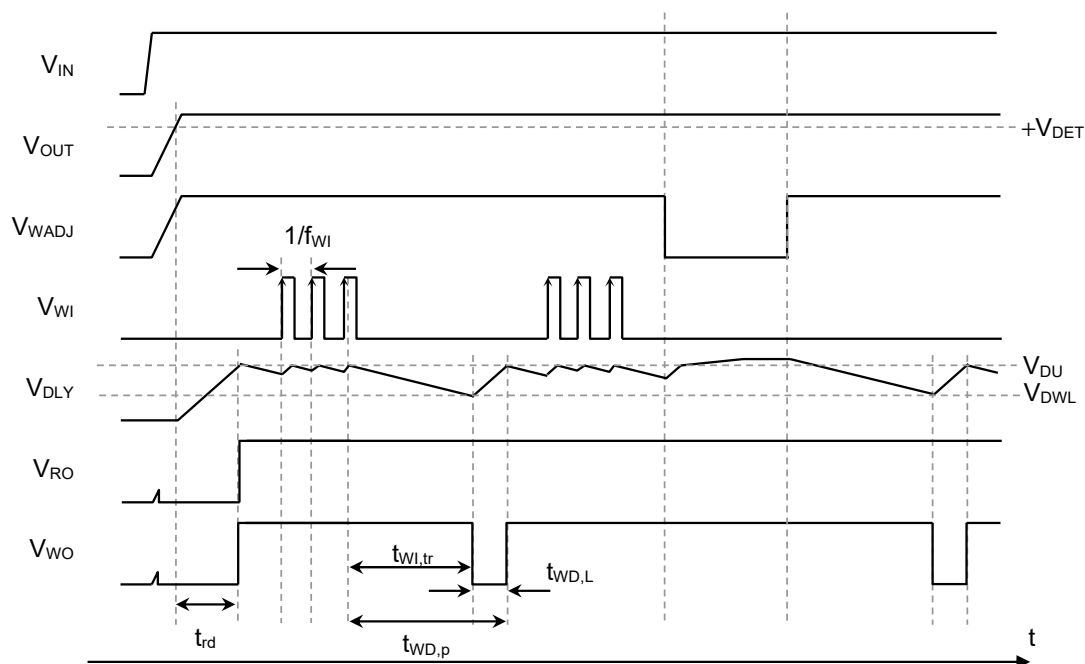
Figure 42 Example of Watchdog Timer Monitoring Operation
