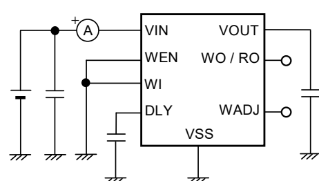
Figure 18 Test Circuit 10
