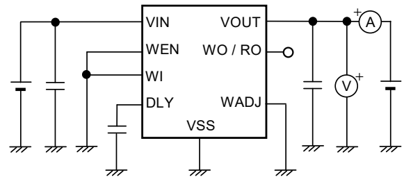
Figure 10 Test Circuit 2
