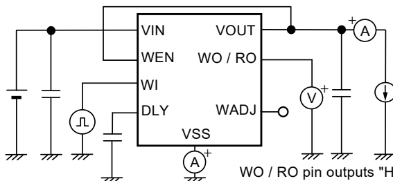
Figure 17 Test Circuit 9
