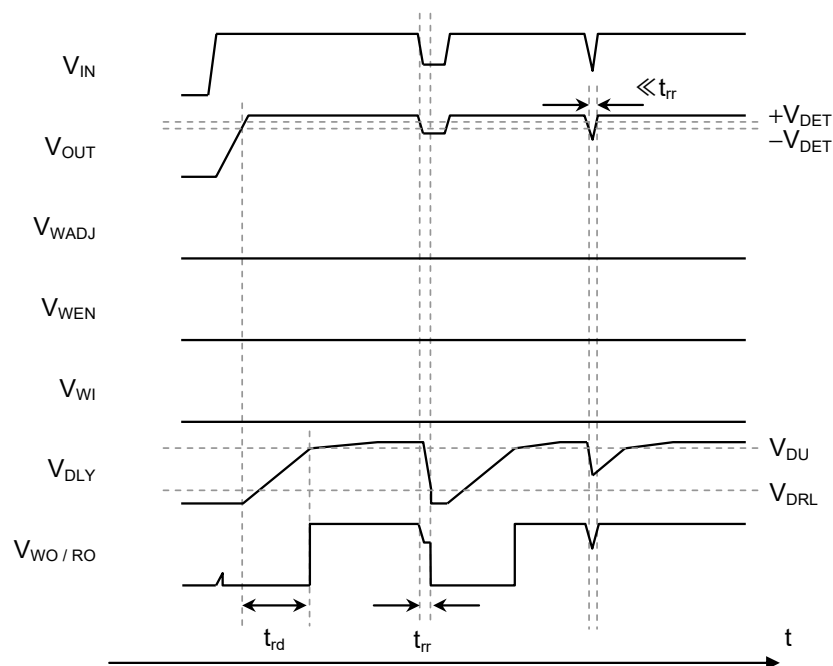
Figure 41 Example of Detector Operation
