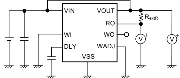
Figure 22 Test Circuit 4
