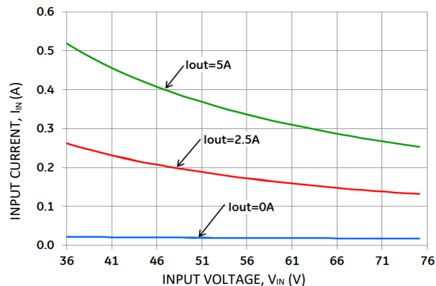
Figure 2. Converter Input Current versus Input Voltage.
