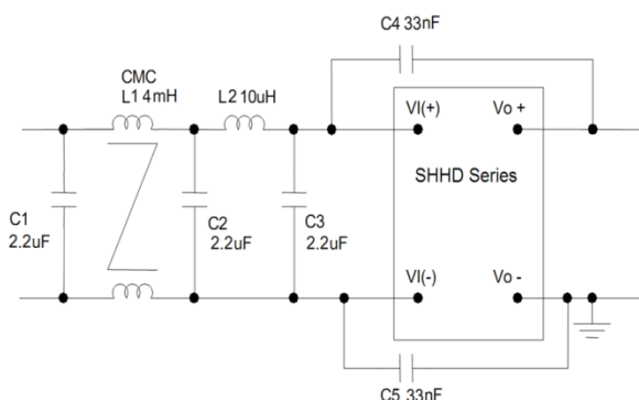
Figure 16. Suggested Configuration for EN55032 Class B.
