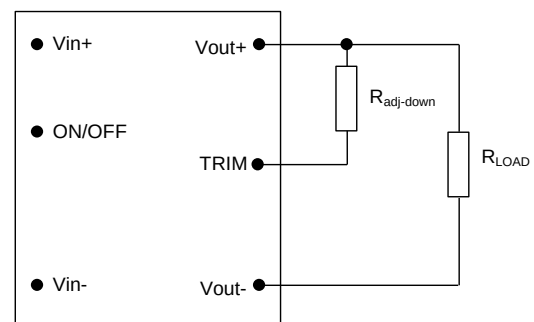
Figure 11. Circuit Configuration to Decrease Output Voltage.
