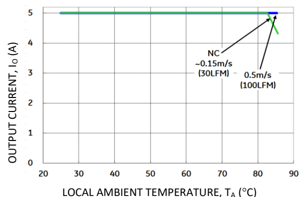
Figure 14. Output Current Derating for the Open Frame SSTW005A0F in the Transverse Orientation; Airflow Direction from Vin(-) to Vin(+); Vin = 48V.
