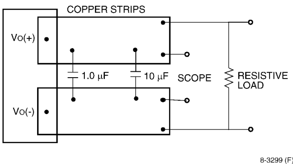
Figure 13. Input Reflected Ripple Current Test Setup.
