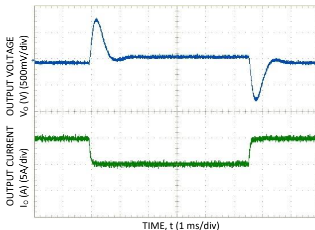
Figure 6. Typical Transient Response to Step Change in Load from 50% to 75% to 50% of Full Load at 48Vdc Input and C_o=470\mu\text{F} Polymer, without -02 option.
