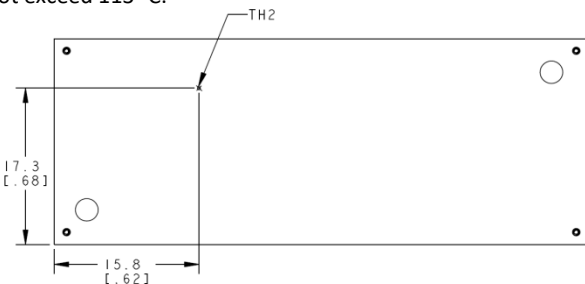
Figure 20. Location of the thermal reference temperature TH_2 for Baseplate module. Do not exceed 110^\circ\text{C} .
