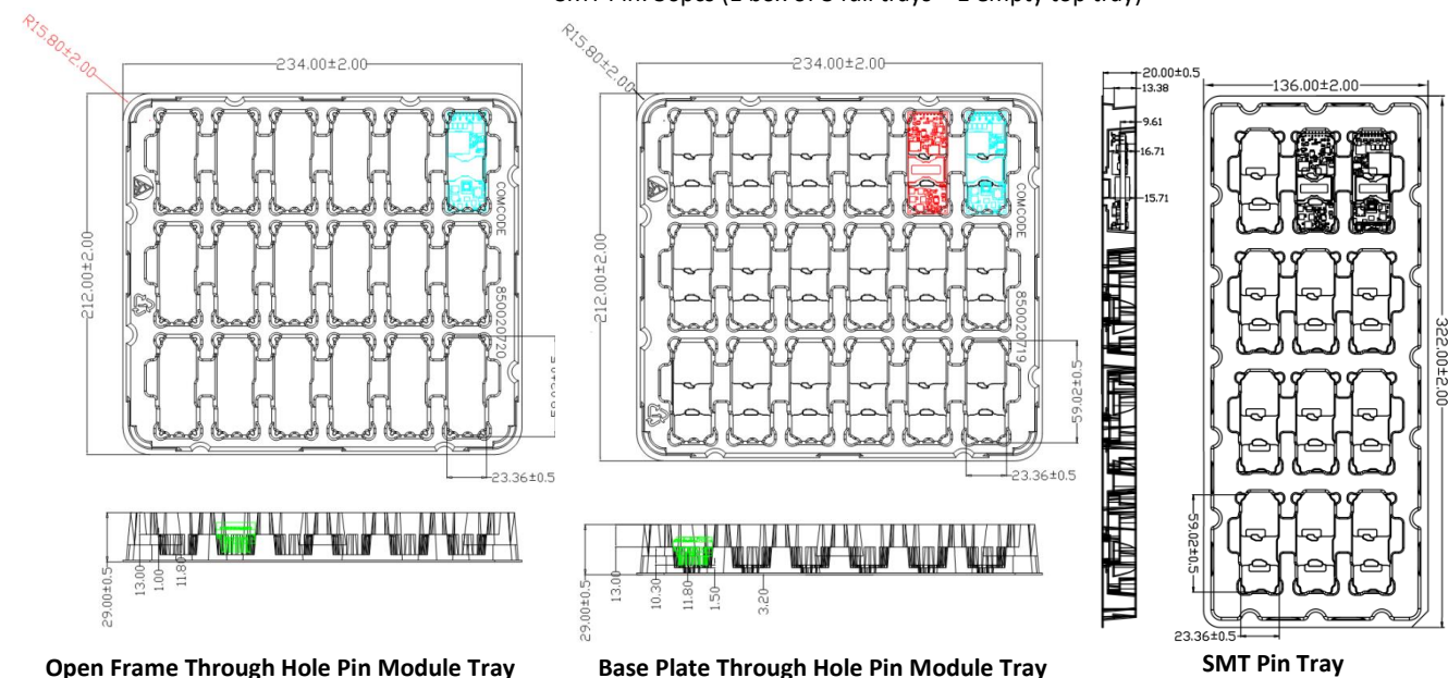
Figure 27. EBDW020 Packaging Tray
