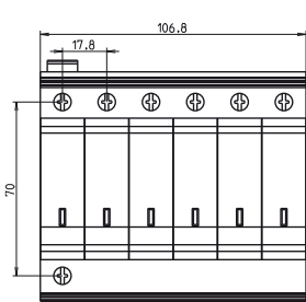
OVR HL 3L 15-440s P TS
