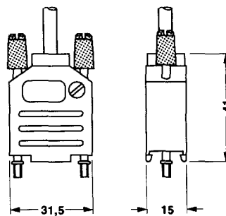
SCT-D-SUB 15-KG
