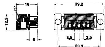
PSC 1,5/5-F
