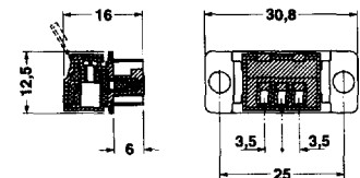
PSC 1,5/5-F
