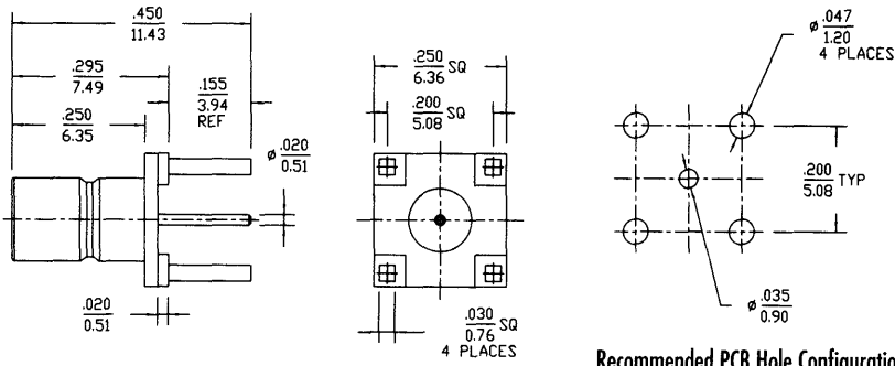
Recommended PCB Hole Configuration
