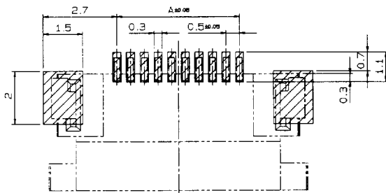
MOUNTING LAYOUT
