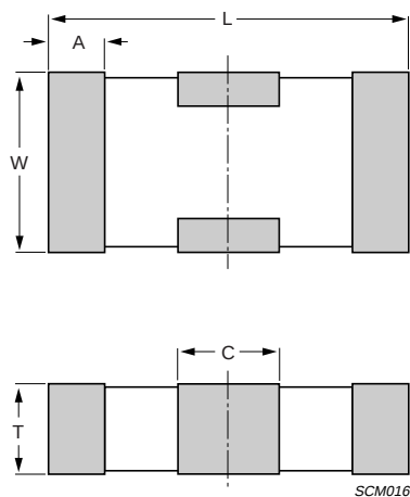
Fig.2. Component outline.
