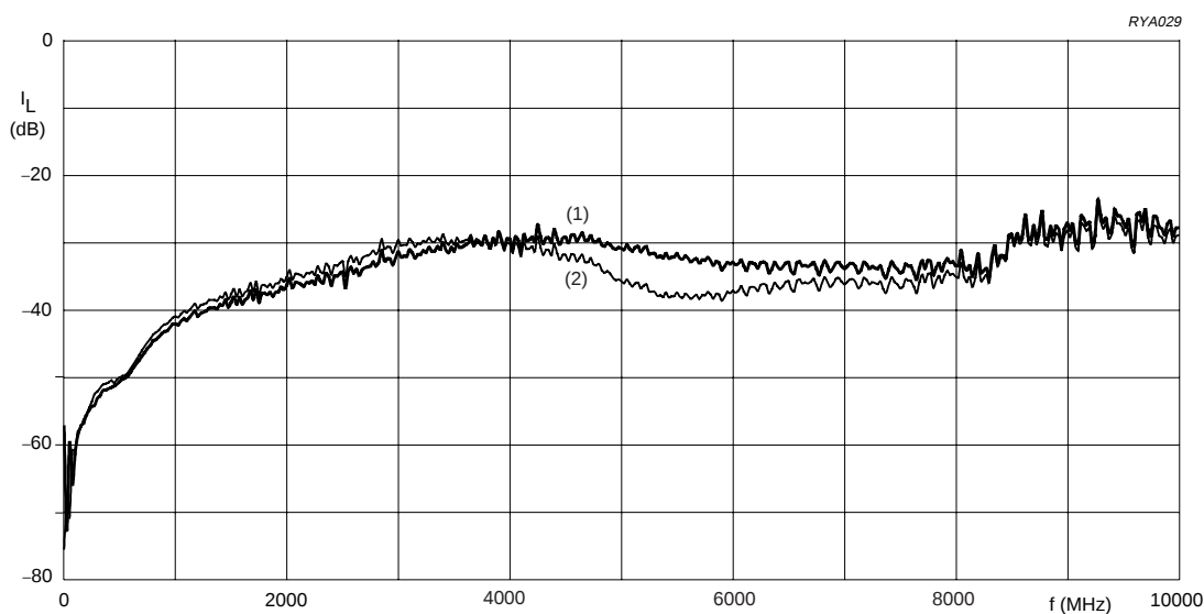
Fig.6 Insertion Loss curves (S21) for X2Y 1812 series.
