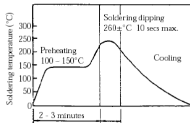
FLOW SOLDERING
