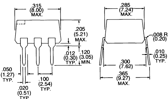
6-Pin DIP Package T-941 thru T-945
