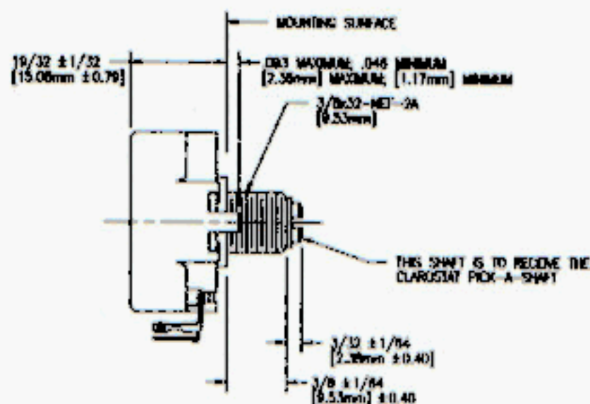
Figure 5 Series A43 Dimensions
