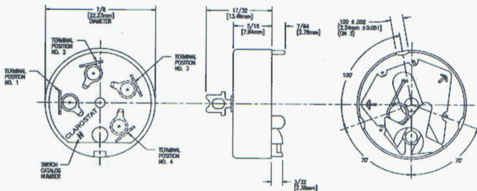
AE Switch Dimensions
