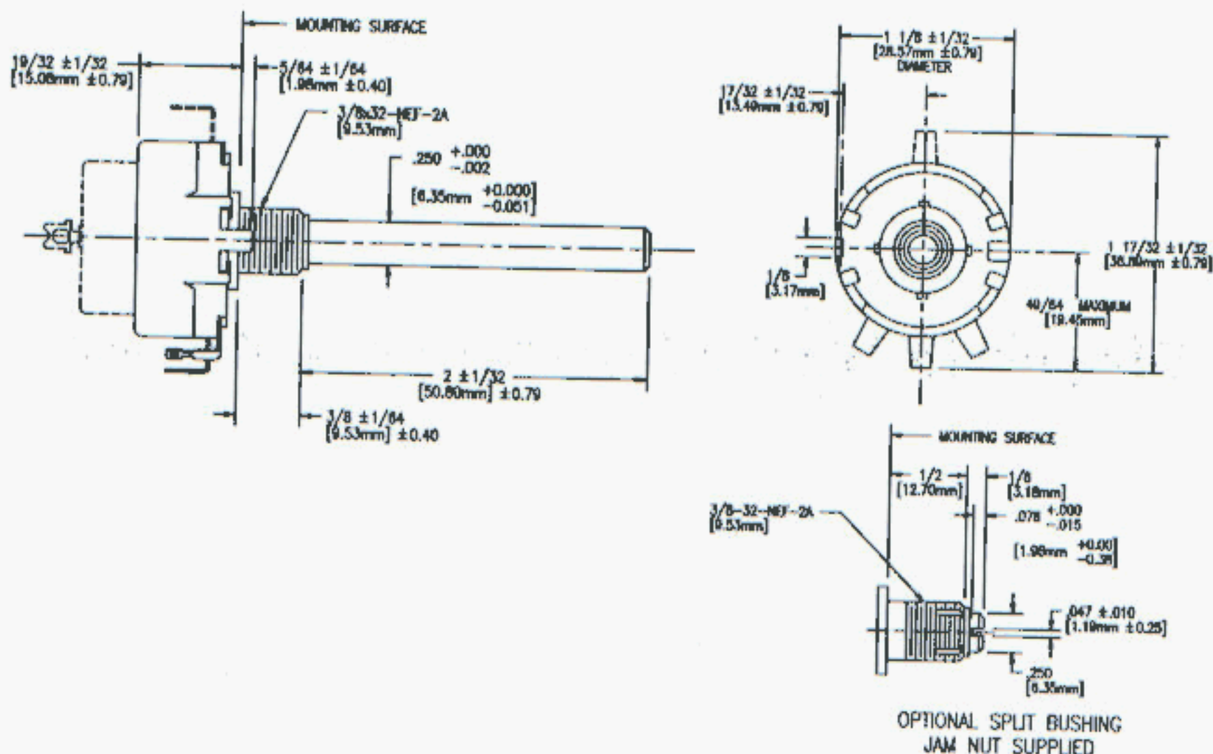
Figure 4 Series 43 Dimensions
